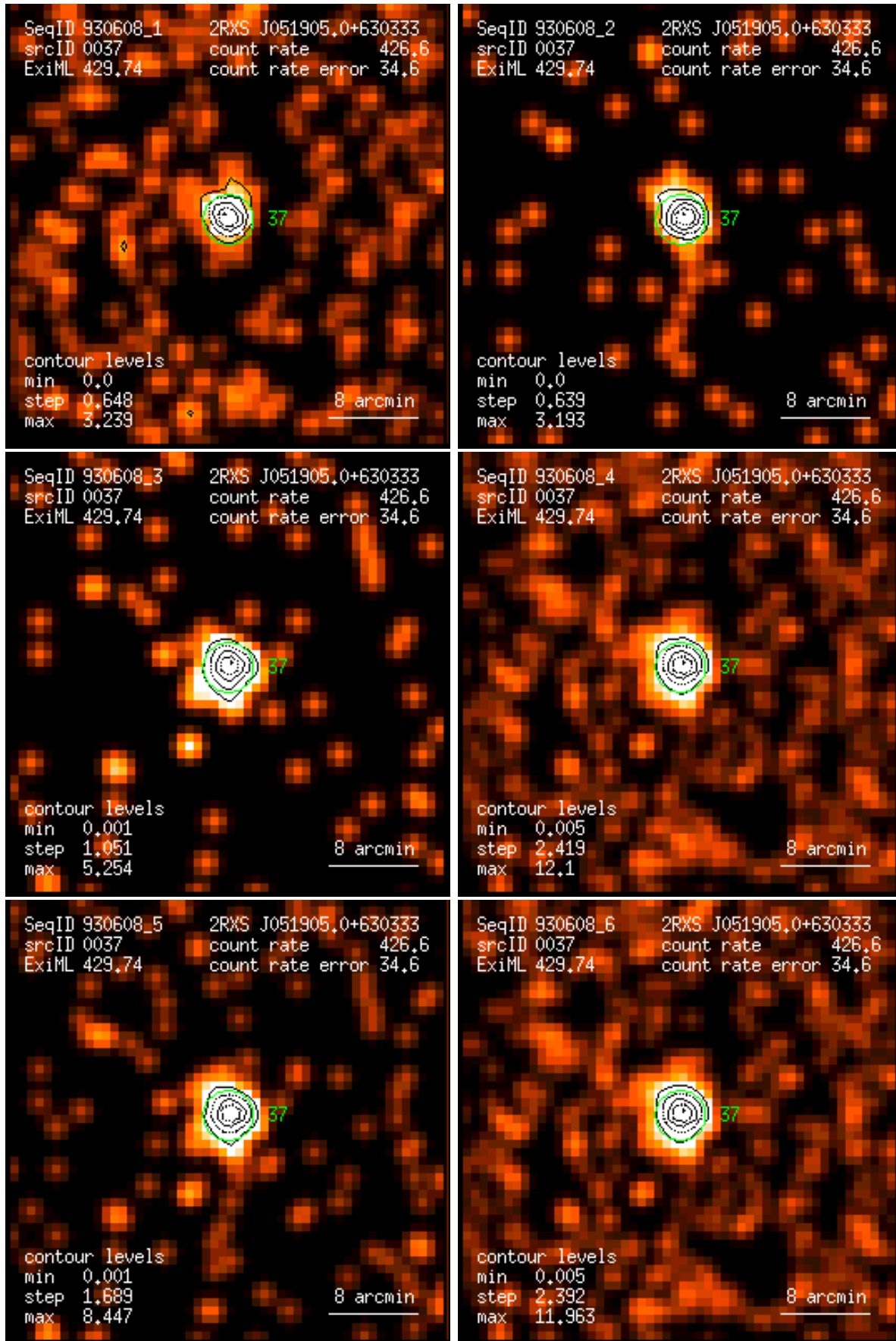
Figure 37: RASS 930608: detection 0037: band rate images, Gaussian filter: (1) PSPC channels 11 – 41, (2) 52 – 90, (3) 91 – 201, (4) 11 – 235, (5) 52 – 201, (6) 11 – 201. Broad band rates in counts/ks. Band rate contour levels in counts/ks/arcmin 2 .
