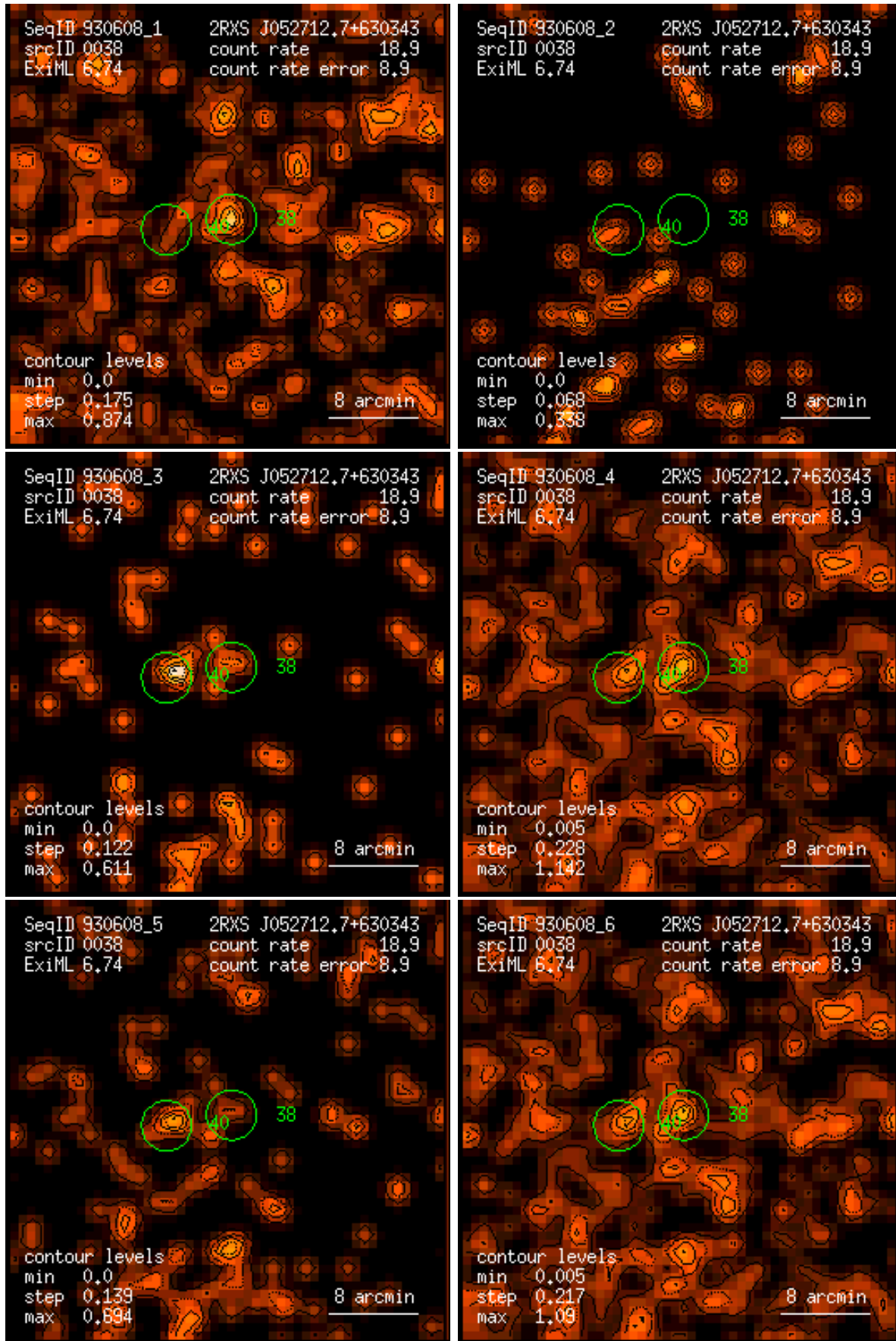
Figure 38: RASS 930608: detection 0038: band rate images, Gaussian filter: (1) PSPC channels 11 – 41, (2) 52 – 90, (3) 91 – 201, (4) 11 – 235, (5) 52 – 201, (6) 11 – 201. Broad band rates in counts/ks. Band rate contour levels in counts/ks/arcmin 2 .
