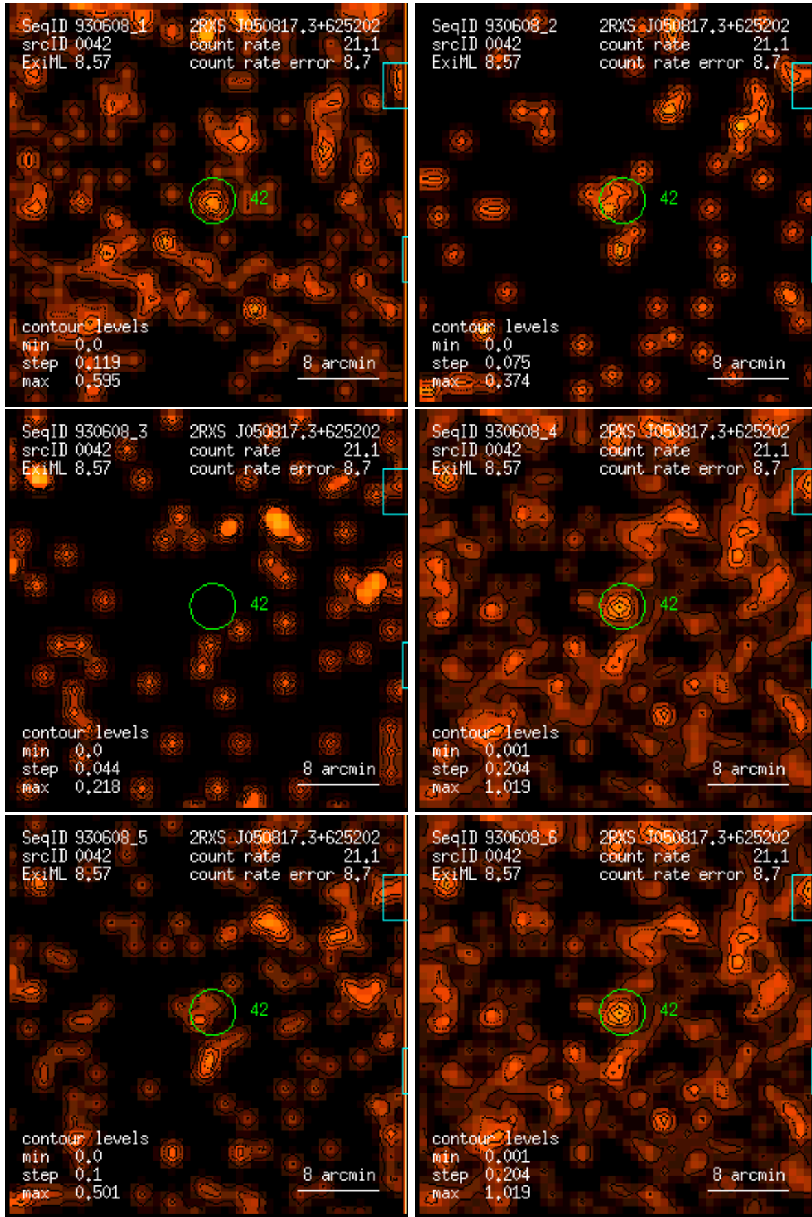
Figure 42: RASS 930608: detection 0042: band rate images, Gaussian filter: (1) PSPC channels 11 – 41, (2) 52 – 90, (3) 91 – 201, (4) 11 – 235, (5) 52 – 201, (6) 11 – 201. Broad band rates in counts/ks. Band rate contour levels in counts/ks/arcmin 2 .
