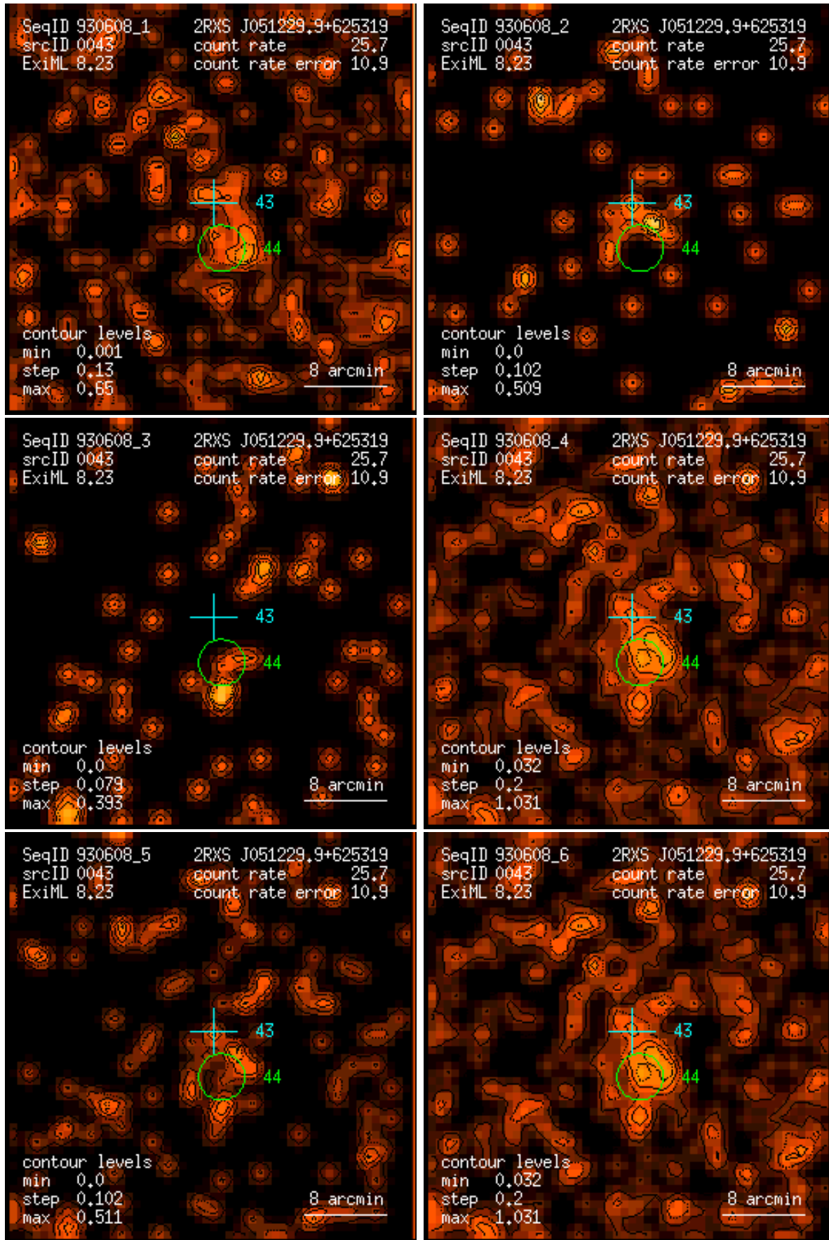
Figure 43: RASS 930608: detection 0043: band rate images, Gaussian filter: (1) PSPC channels 11 – 41, (2) 52 – 90, (3) 91 – 201, (4) 11 – 235, (5) 52 – 201, (6) 11 – 201. Broad band rates in counts/ks. Band rate contour levels in counts/ks/arcmin 2 .
