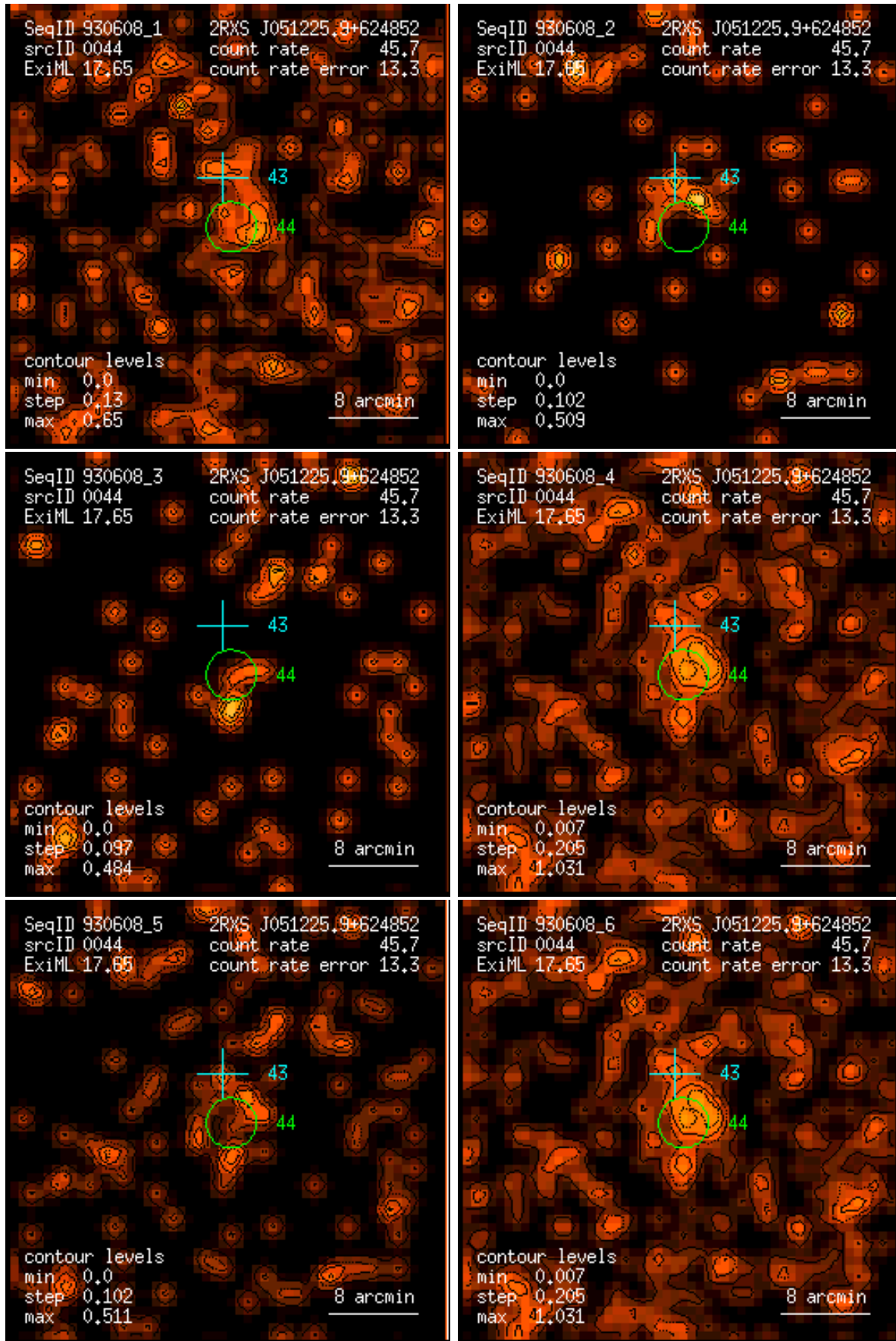
Figure 44: RASS 930608: detection 0044: band rate images, Gaussian filter: (1) PSPC channels 11 – 41, (2) 52 – 90, (3) 91 – 201, (4) 11 – 235, (5) 52 – 201, (6) 11 – 201. Broad band rates in counts/ks. Band rate contour levels in counts/ks/arcmin 2 .
