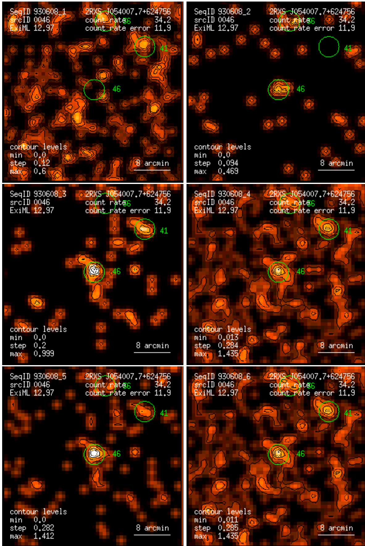
Figure 46: RASS 930608: detection 0046: band rate images, Gaussian filter: (1) PSPC channels 11 – 41, (2) 52 – 90, (3) 91 – 201, (4) 11 – 235, (5) 52 – 201, (6) 11 – 201. Broad band rates in counts/ks. Band rate contour levels in counts/ks/arcmin 2 .
