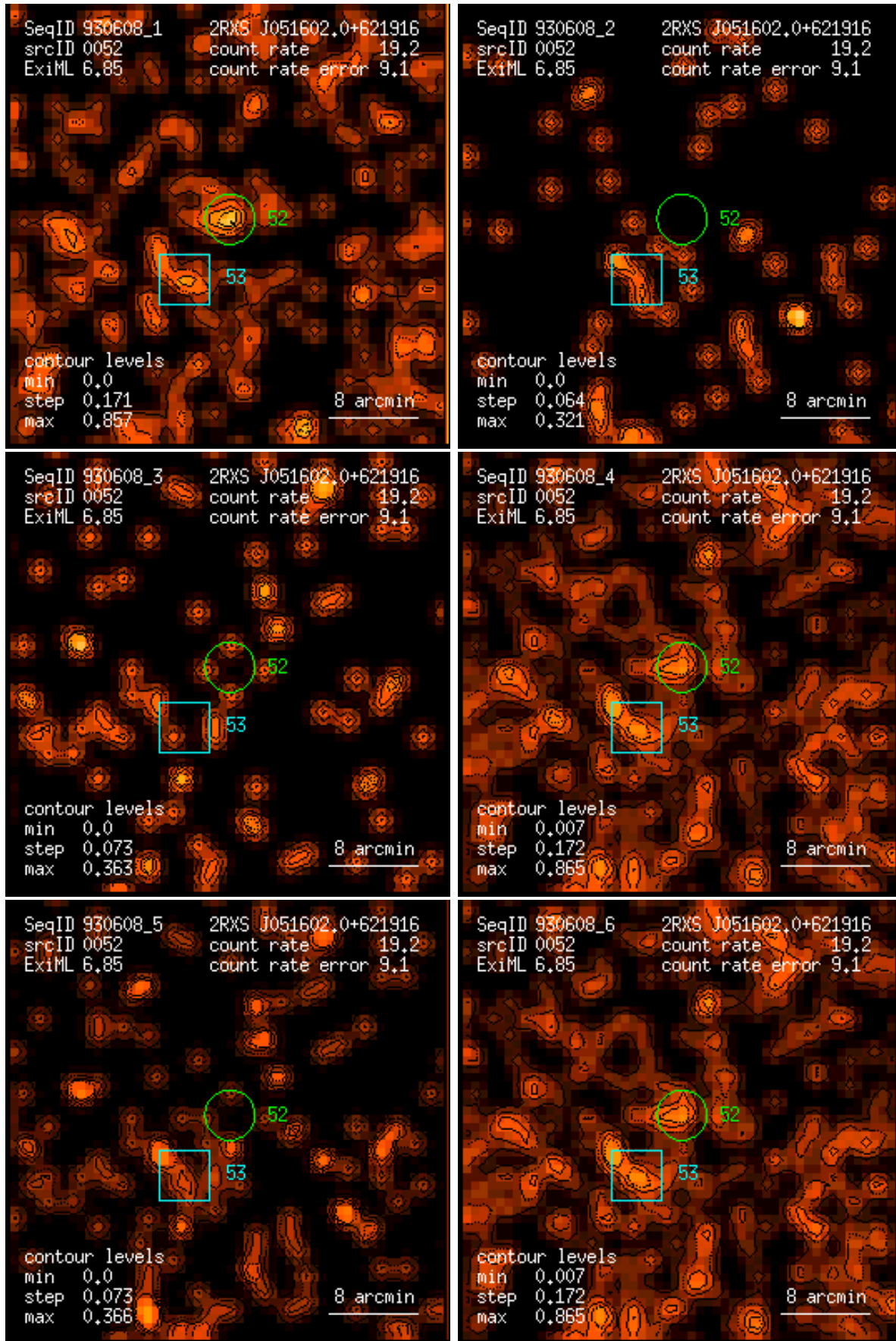
Figure 52: RASS 930608: detection 0052: band rate images, Gaussian filter: (1) PSPC channels 11 – 41, (2) 52 – 90, (3) 91 – 201, (4) 11 – 235, (5) 52 – 201, (6) 11 – 201. Broad band rates in counts/ks. Band rate contour levels in counts/ks/arcmin 2 .
