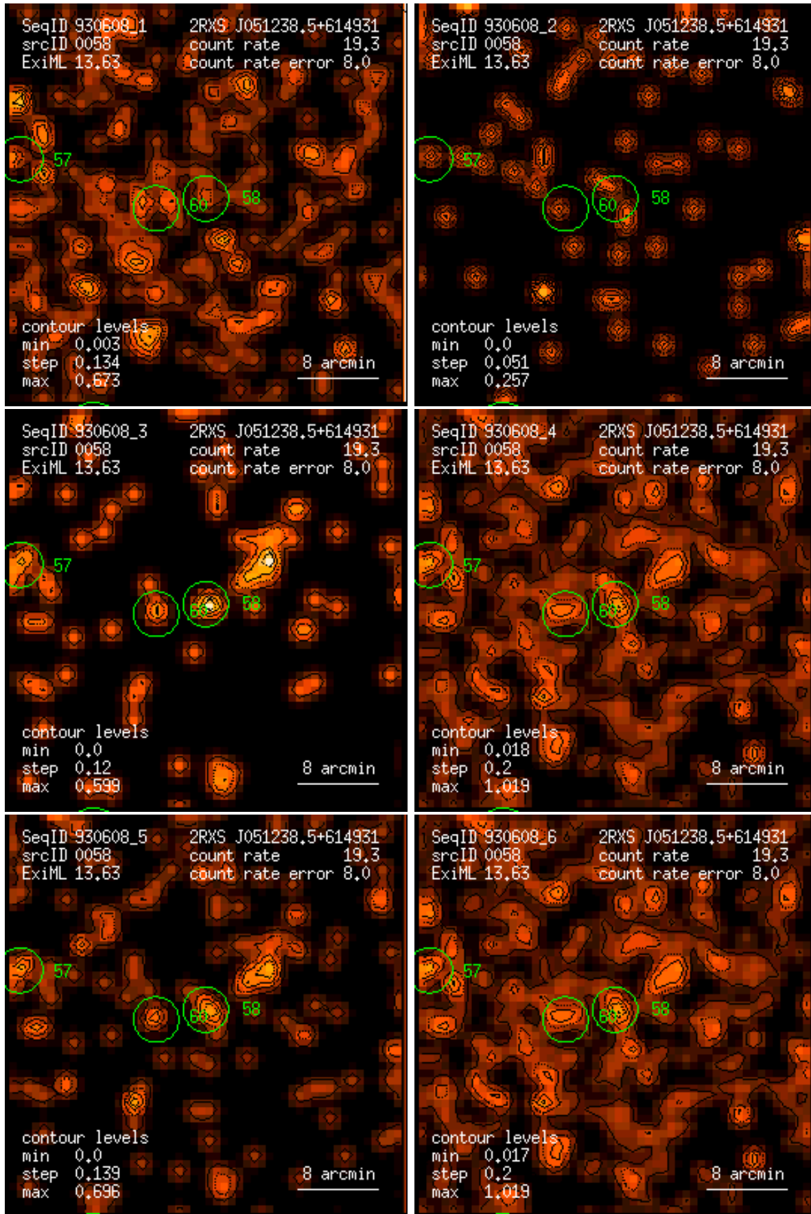
Figure 58: RASS 930608: detection 0058: band rate images, Gaussian filter: (1) PSPC channels 11 – 41, (2) 52 – 90, (3) 91 – 201, (4) 11 – 235, (5) 52 – 201, (6) 11 – 201. Broad band rates in counts/ks. Band rate contour levels in counts/ks/arcmin 2 .
