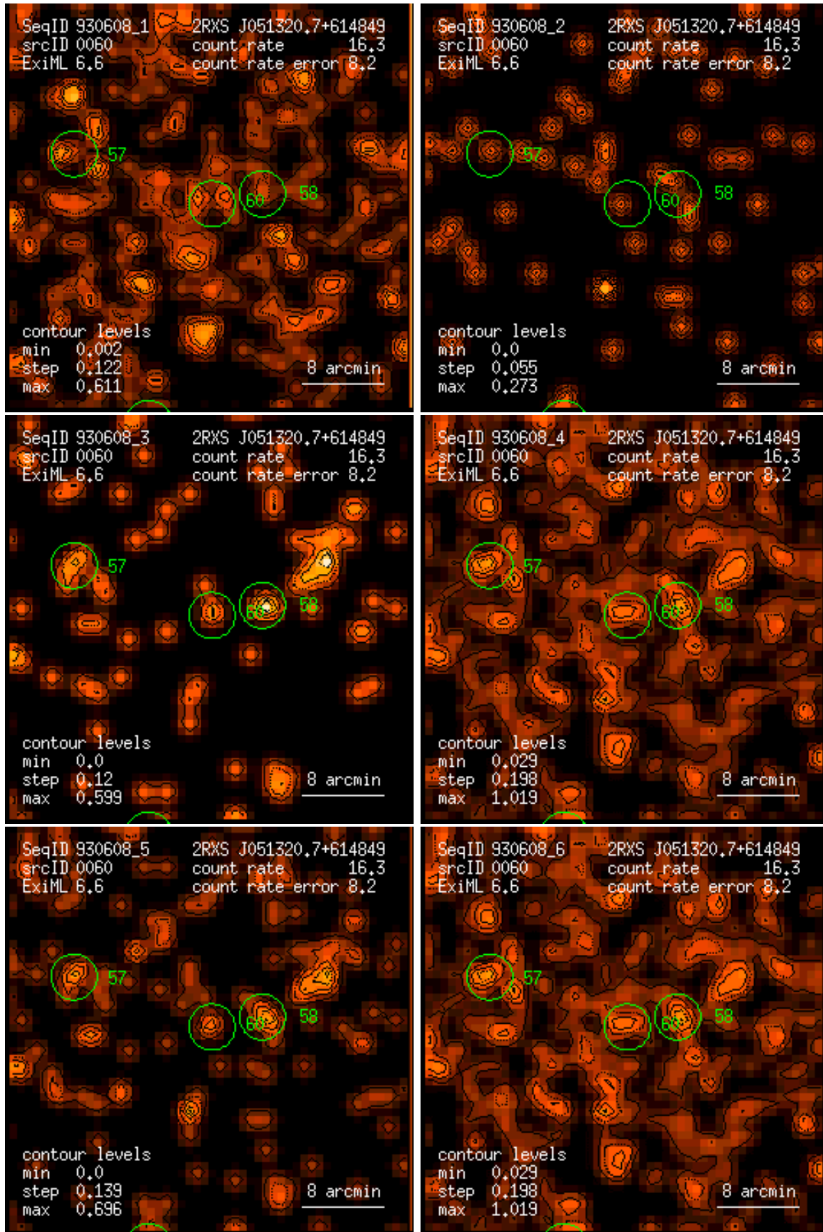
Figure 60: RASS 930608: detection 0060: band rate images, Gaussian filter: (1) PSPC channels 11 – 41, (2) 52 – 90, (3) 91 – 201, (4) 11 – 235, (5) 52 – 201, (6) 11 – 201. Broad band rates in counts/ks. Band rate contour levels in counts/ks/arcmin 2 .
