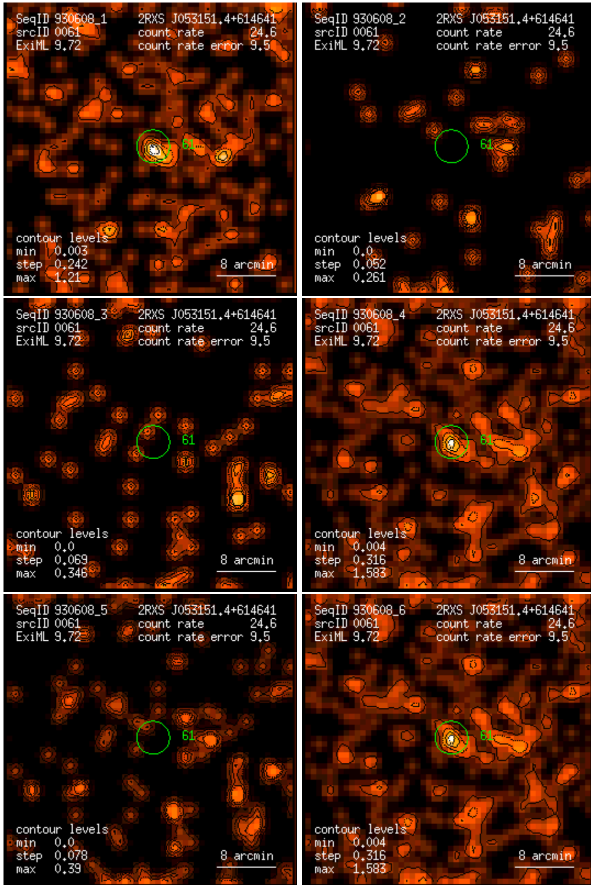
Figure 61: RASS 930608: detection 0061: band rate images, Gaussian filter: (1) PSPC channels 11 – 41, (2) 52 – 90, (3) 91 – 201, (4) 11 – 235, (5) 52 – 201, (6) 11 – 201. Broad band rates in counts/ks. Band rate contour levels in counts/ks/arcmin 2 .
