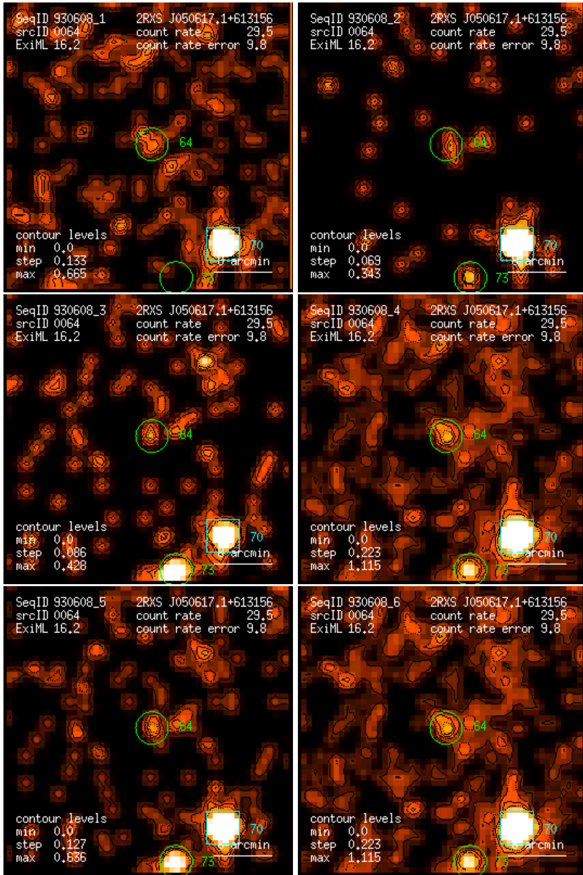
Figure 64: RASS 930608: detection 0064: band rate images, Gaussian filter: (1) PSPC channels 11 – 41, (2) 52 – 90, (3) 91 – 201, (4) 11 – 235, (5) 52 – 201, (6) 11 – 201. Broad band rates in counts/ks. Band rate contour levels in counts/ks/arcmin 2 .
