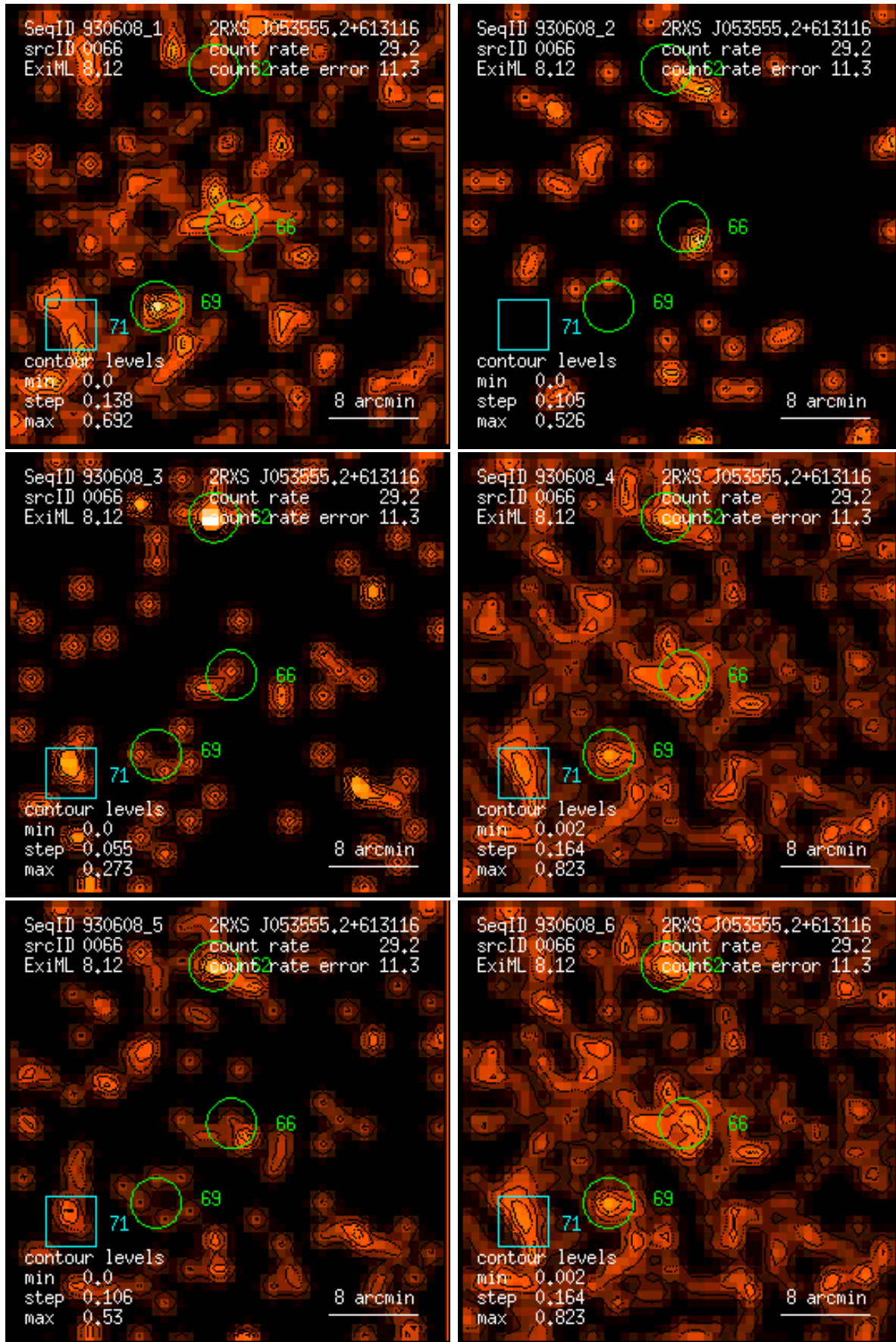
Figure 66: RASS 930608: detection 0066: band rate images, Gaussian filter: (1) PSPC channels 11 – 41, (2) 52 – 90, (3) 91 – 201, (4) 11 – 235, (5) 52 – 201, (6) 11 – 201. Broad band rates in counts/ks. Band rate contour levels in counts/ks/arcmin 2 .
