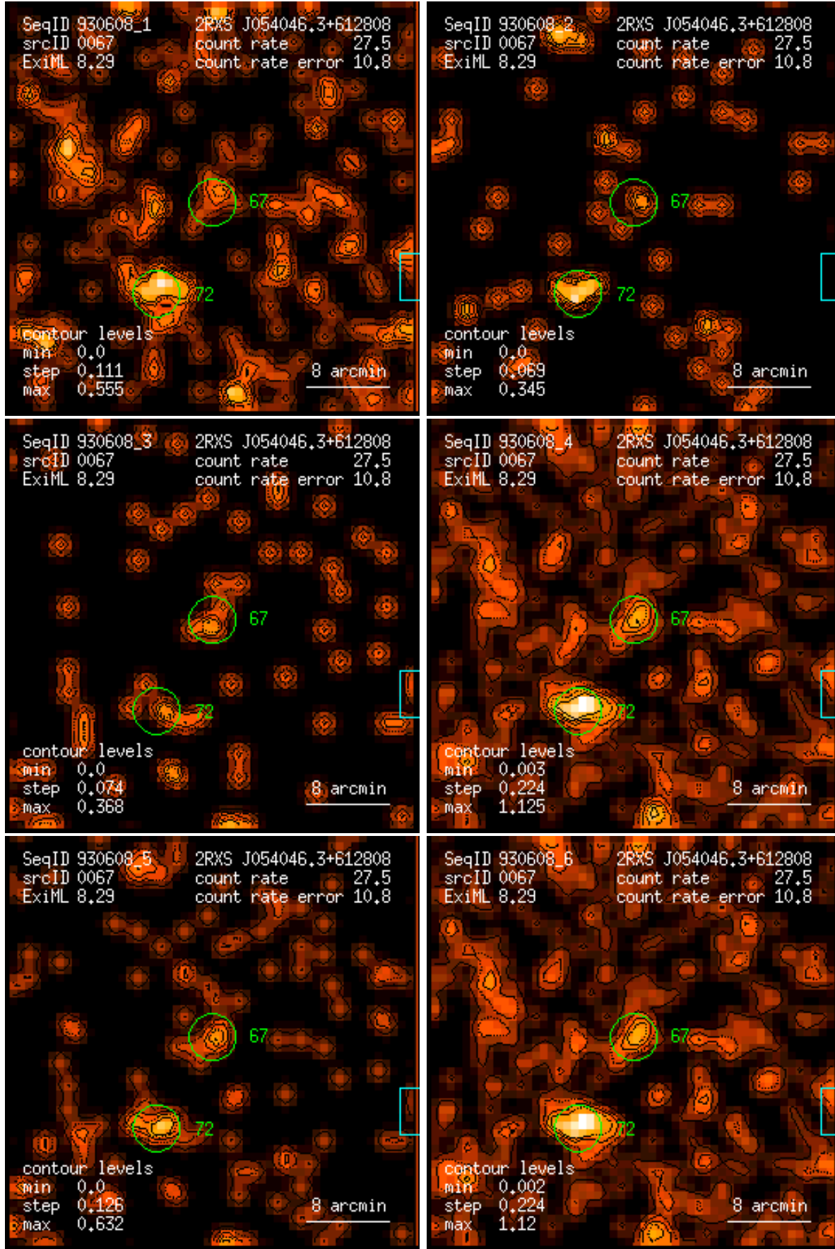
Figure 67: RASS 930608: detection 0067: band rate images, Gaussian filter: (1) PSPC channels 11 – 41, (2) 52 – 90, (3) 91 – 201, (4) 11 – 235, (5) 52 – 201, (6) 11 – 201. Broad band rates in counts/ks. Band rate contour levels in counts/ks/arcmin 2 .
