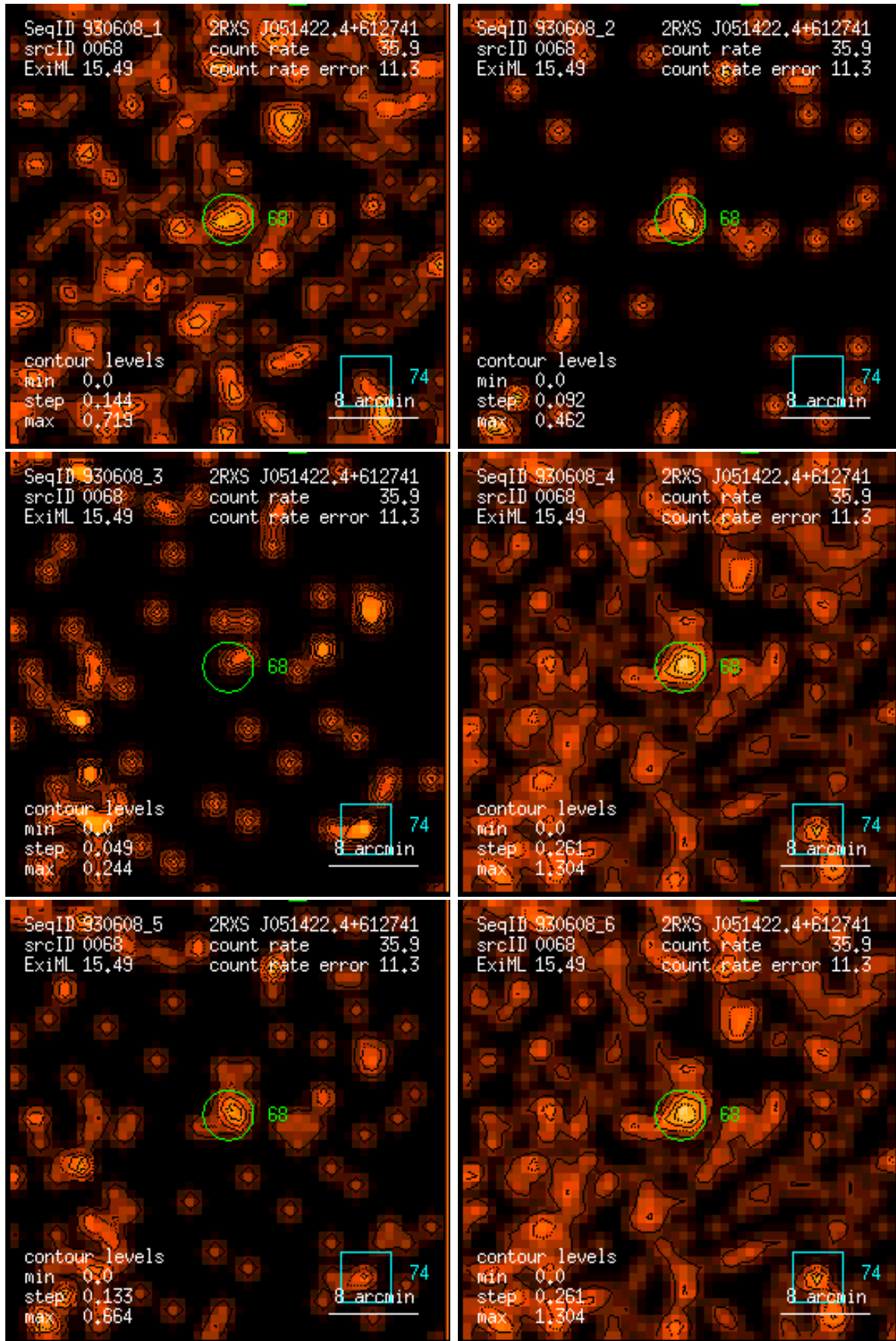
Figure 68: RASS 930608: detection 0068: band rate images, Gaussian filter: (1) PSPC channels 11 – 41, (2) 52 – 90, (3) 91 – 201, (4) 11 – 235, (5) 52 – 201, (6) 11 – 201. Broad band rates in counts/ks. Band rate contour levels in counts/ks/arcmin 2 .
