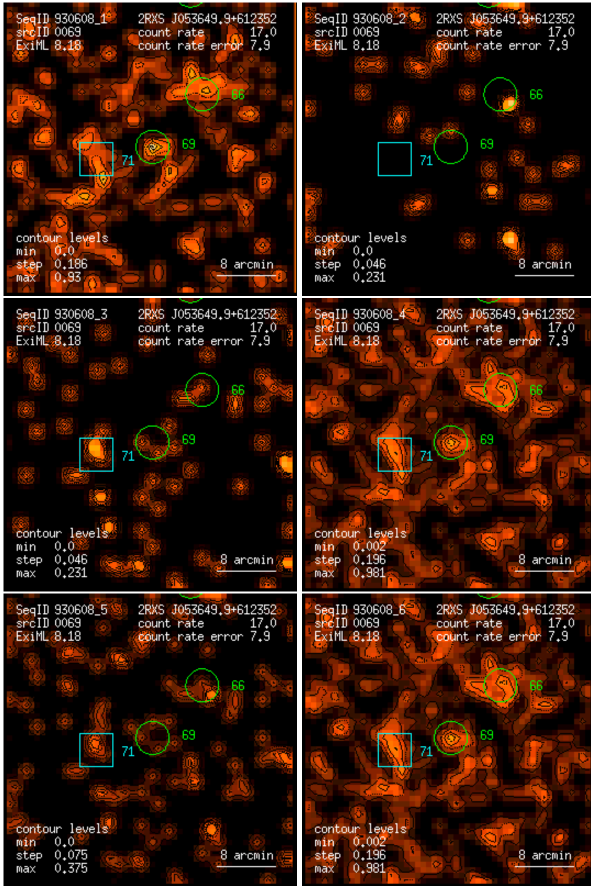
Figure 69: RASS 930608: detection 0069: band rate images, Gaussian filter: (1) PSPC channels 11 – 41, (2) 52 – 90, (3) 91 – 201, (4) 11 – 235, (5) 52 – 201, (6) 11 – 201. Broad band rates in counts/ks. Band rate contour levels in counts/ks/arcmin 2 .
