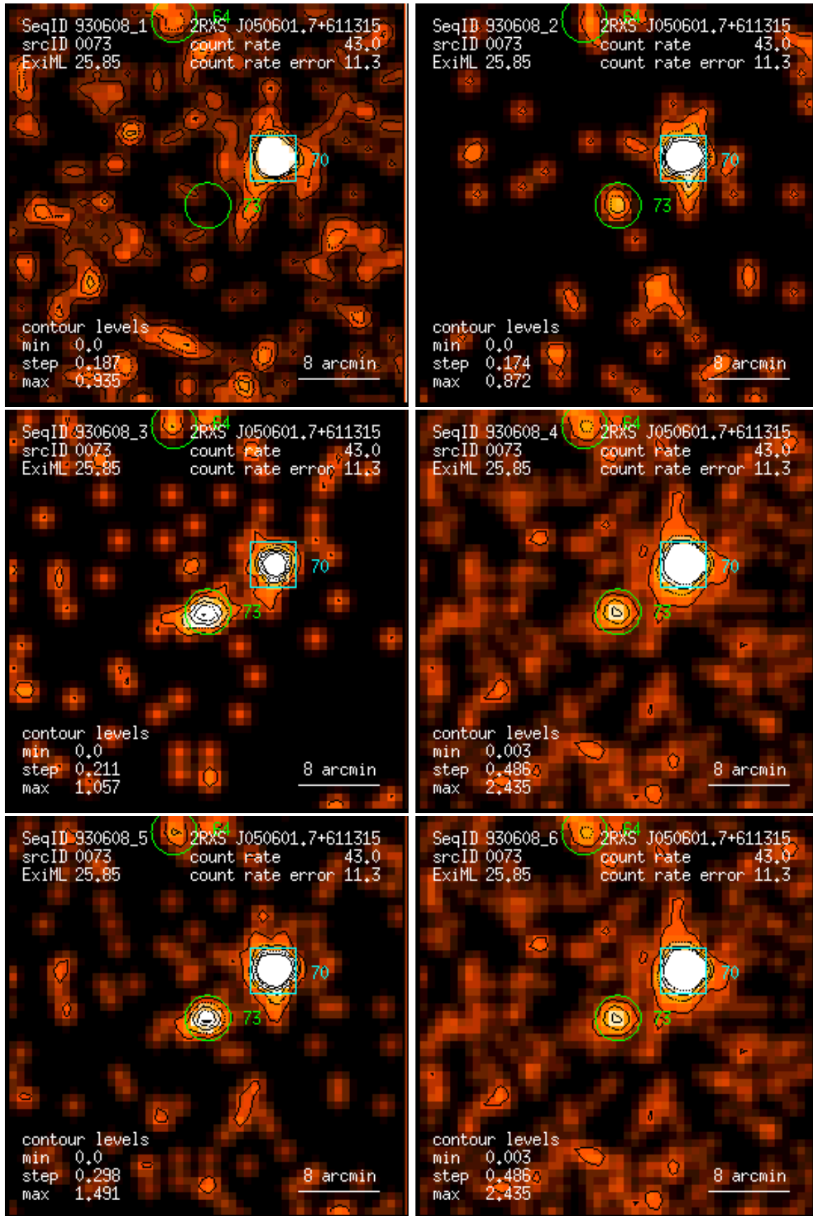
Figure 73: RASS 930608: detection 0073: band rate images, Gaussian filter: (1) PSPC channels 11 – 41, (2) 52 – 90, (3) 91 – 201, (4) 11 – 235, (5) 52 – 201, (6) 11 – 201. Broad band rates in counts/ks. Band rate contour levels in counts/ks/arcmin 2 .
