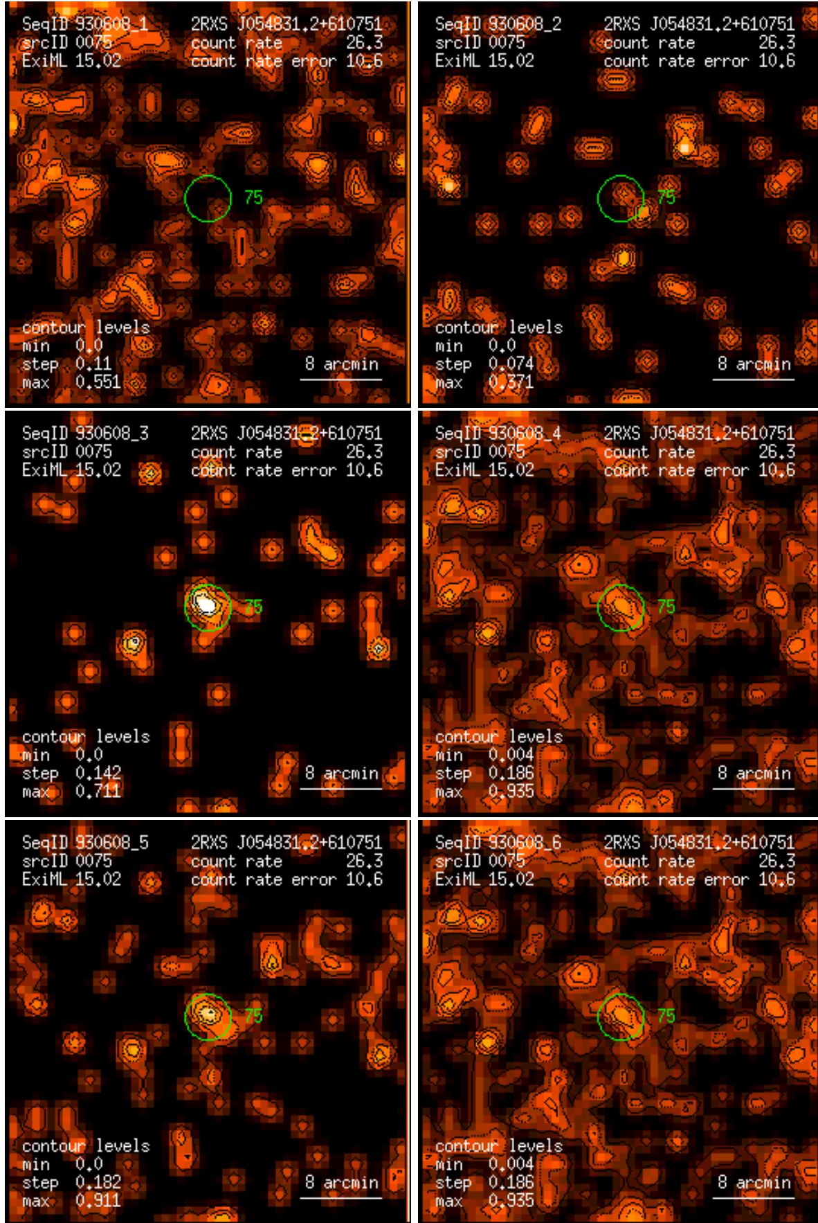
Figure 75: RASS 930608: detection 0075: band rate images, Gaussian filter: (1) PSPC channels 11 – 41, (2) 52 – 90, (3) 91 – 201, (4) 11 – 235, (5) 52 – 201, (6) 11 – 201. Broad band rates in counts/ks. Band rate contour levels in counts/ks/arcmin 2 .
