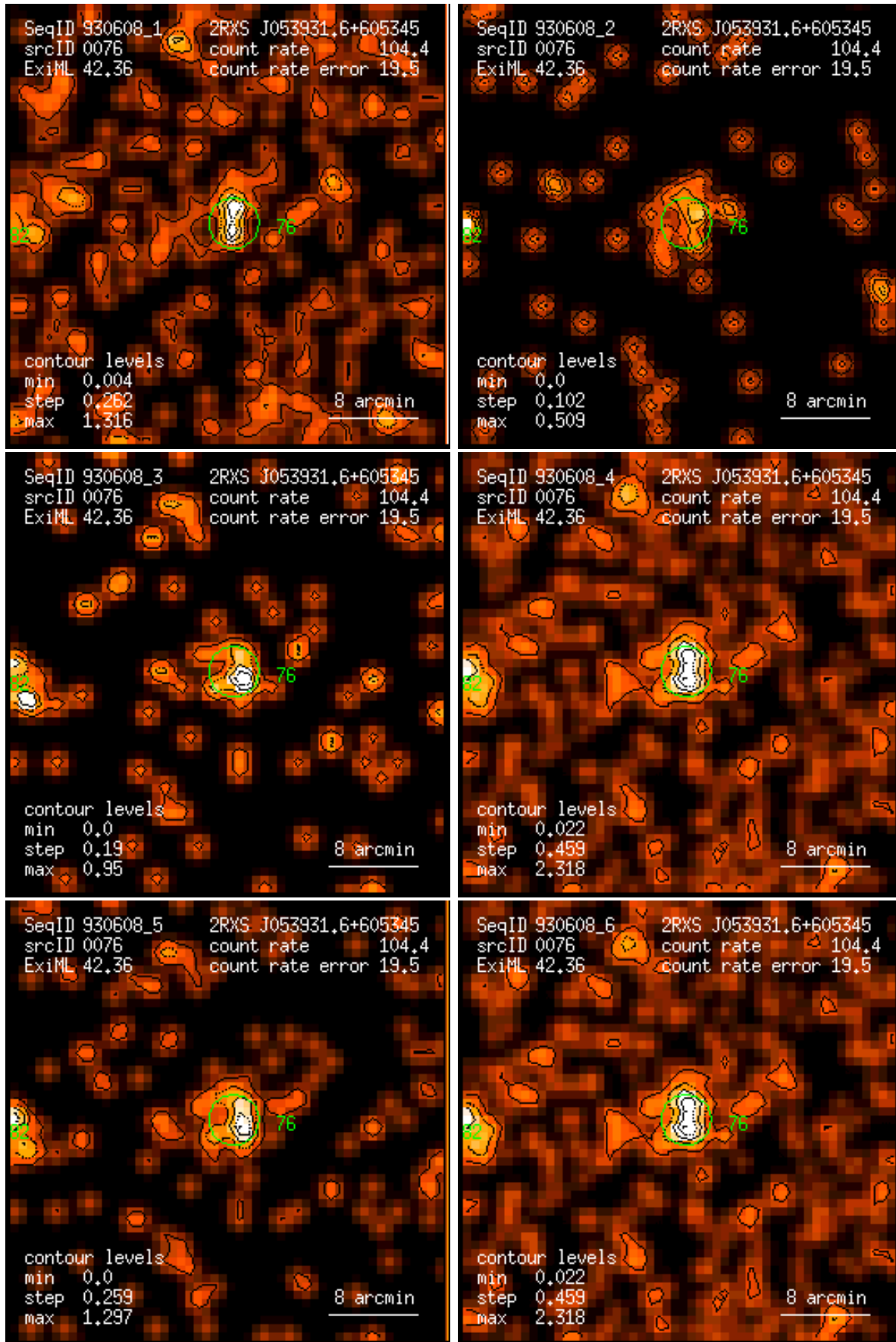
Figure 76: RASS 930608: detection 0076: band rate images, Gaussian filter: (1) PSPC channels 11 – 41, (2) 52 – 90, (3) 91 – 201, (4) 11 – 235, (5) 52 – 201, (6) 11 – 201. Broad band rates in counts/ks. Band rate contour levels in counts/ks/arcmin 2 .
