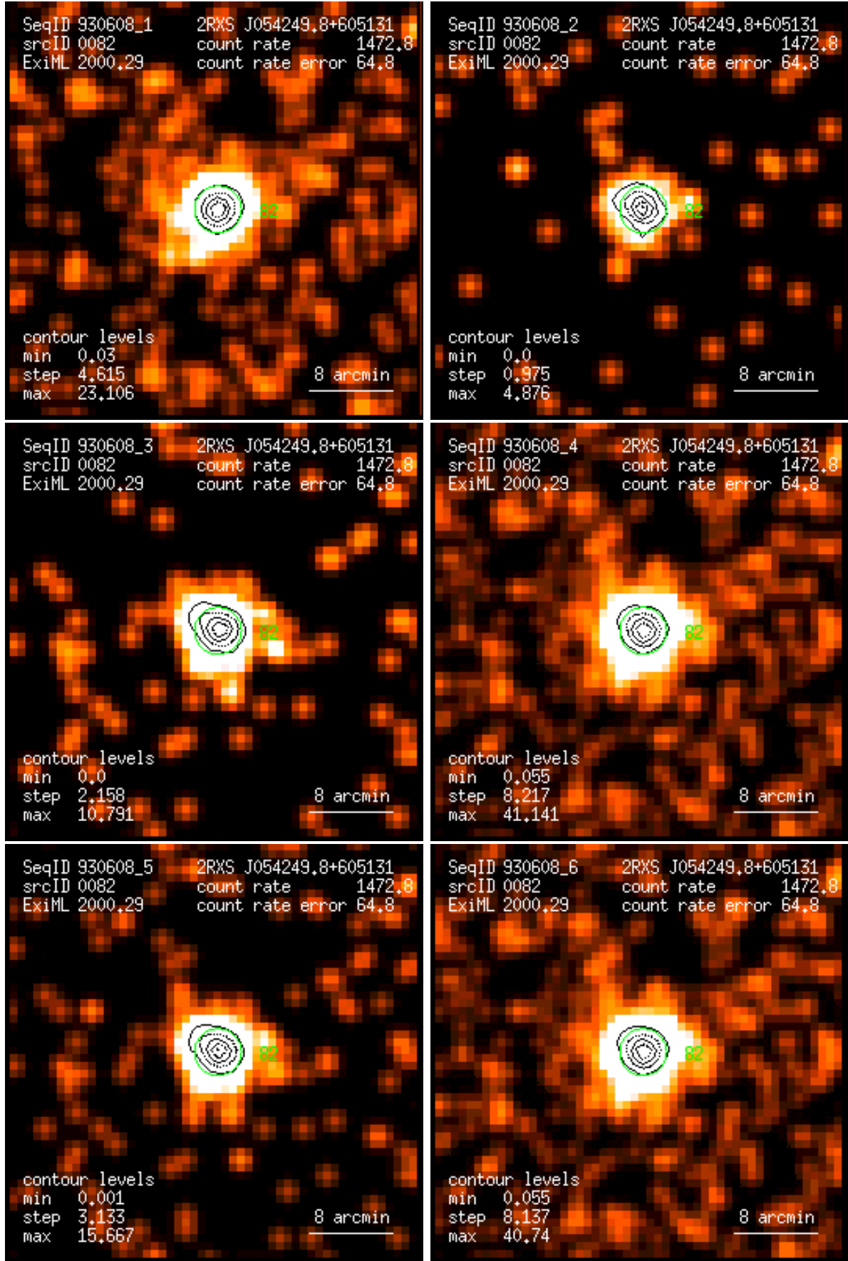
Figure 82: RASS 930608: detection 0082: band rate images, Gaussian filter: (1) PSPC channels 11 – 41, (2) 52 – 90, (3) 91 – 201, (4) 11 – 235, (5) 52 – 201, (6) 11 – 201. Broad band rates in counts/ks. Band rate contour levels in counts/ks/arcmin 2 .
