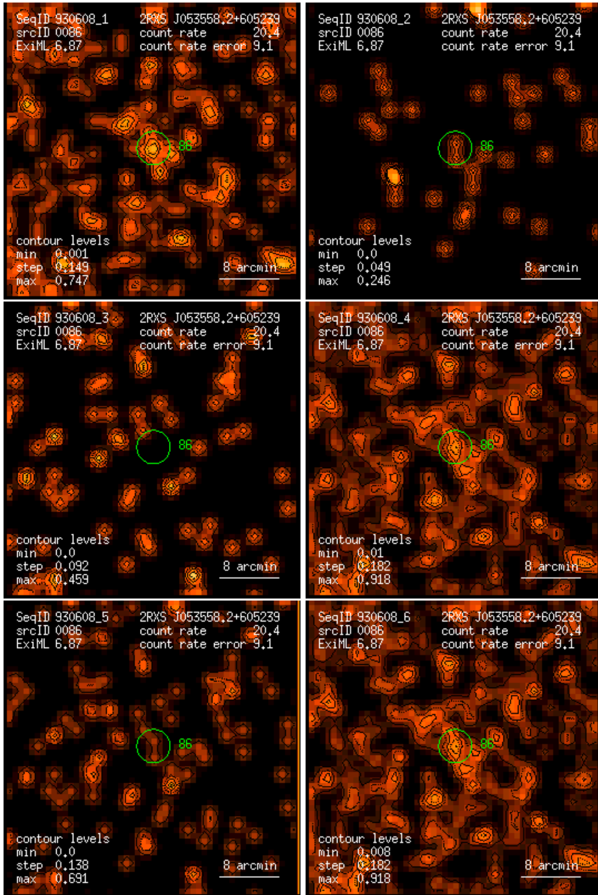
Figure 86: RASS 930608: detection 0086: band rate images, Gaussian filter: (1) PSPC channels 11 – 41, (2) 52 – 90, (3) 91 – 201, (4) 11 – 235, (5) 52 – 201, (6) 11 – 201. Broad band rates in counts/ks. Band rate contour levels in counts/ks/arcmin 2 .
