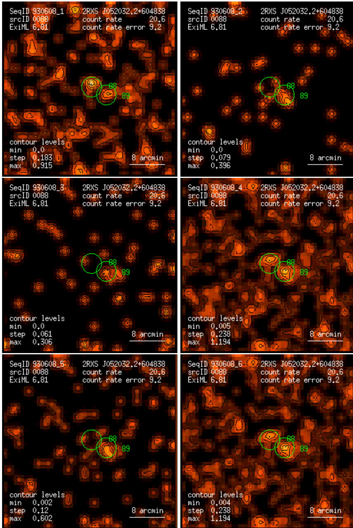
Figure 88: RASS 930608: detection 0088: band rate images, Gaussian filter: (1) PSPC channels 11 – 41, (2) 52 – 90, (3) 91 – 201, (4) 11 – 235, (5) 52 – 201, (6) 11 – 201. Broad band rates in counts/ks. Band rate contour levels in counts/ks/arcmin 2 .
