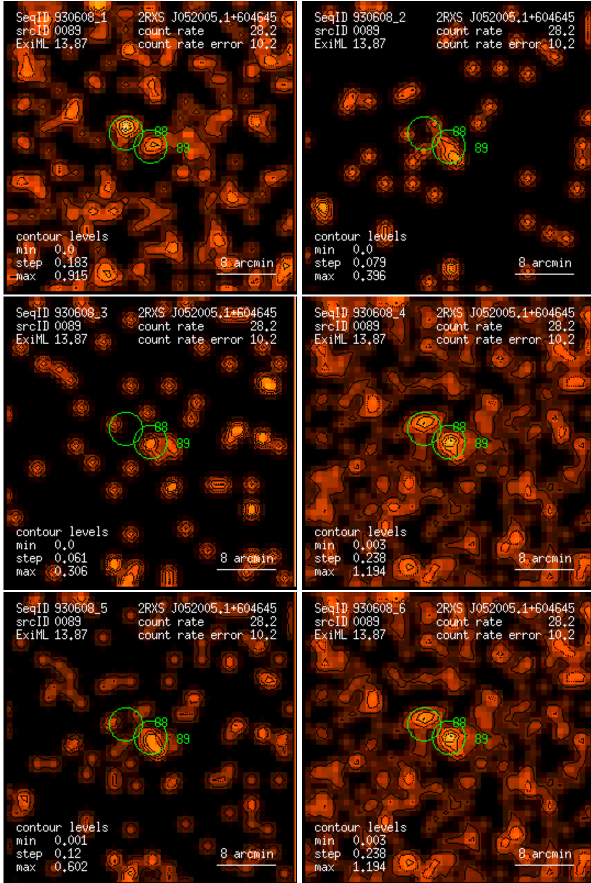
Figure 89: RASS 930608: detection 0089: band rate images, Gaussian filter: (1) PSPC channels 11 – 41, (2) 52 – 90, (3) 91 – 201, (4) 11 – 235, (5) 52 – 201, (6) 11 – 201. Broad band rates in counts/ks. Band rate contour levels in counts/ks/arcmin 2 .
