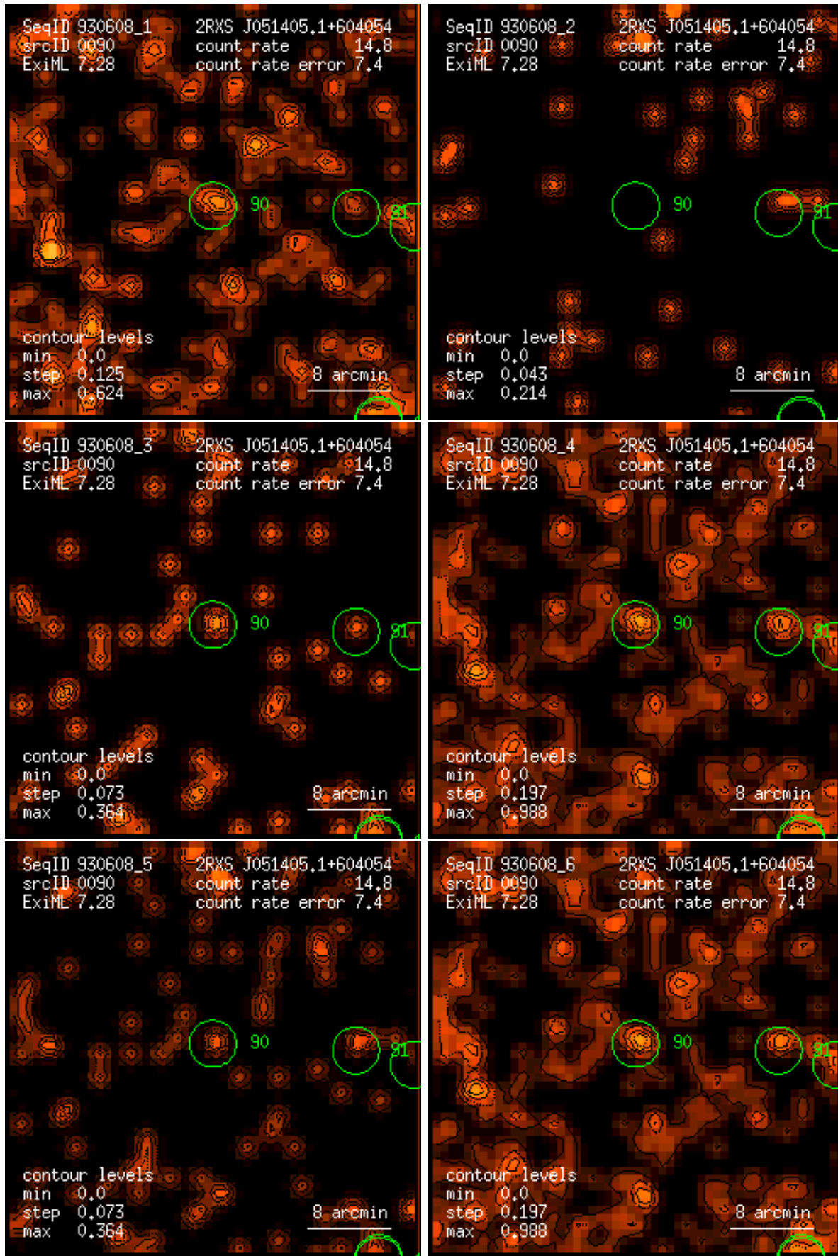
Figure 90: RASS 930608: detection 0090: band rate images, Gaussian filter: (1) PSPC channels 11 – 41, (2) 52 – 90, (3) 91 – 201, (4) 11 – 235, (5) 52 – 201, (6) 11 – 201. Broad band rates in counts/ks. Band rate contour levels in counts/ks/arcmin 2 .
