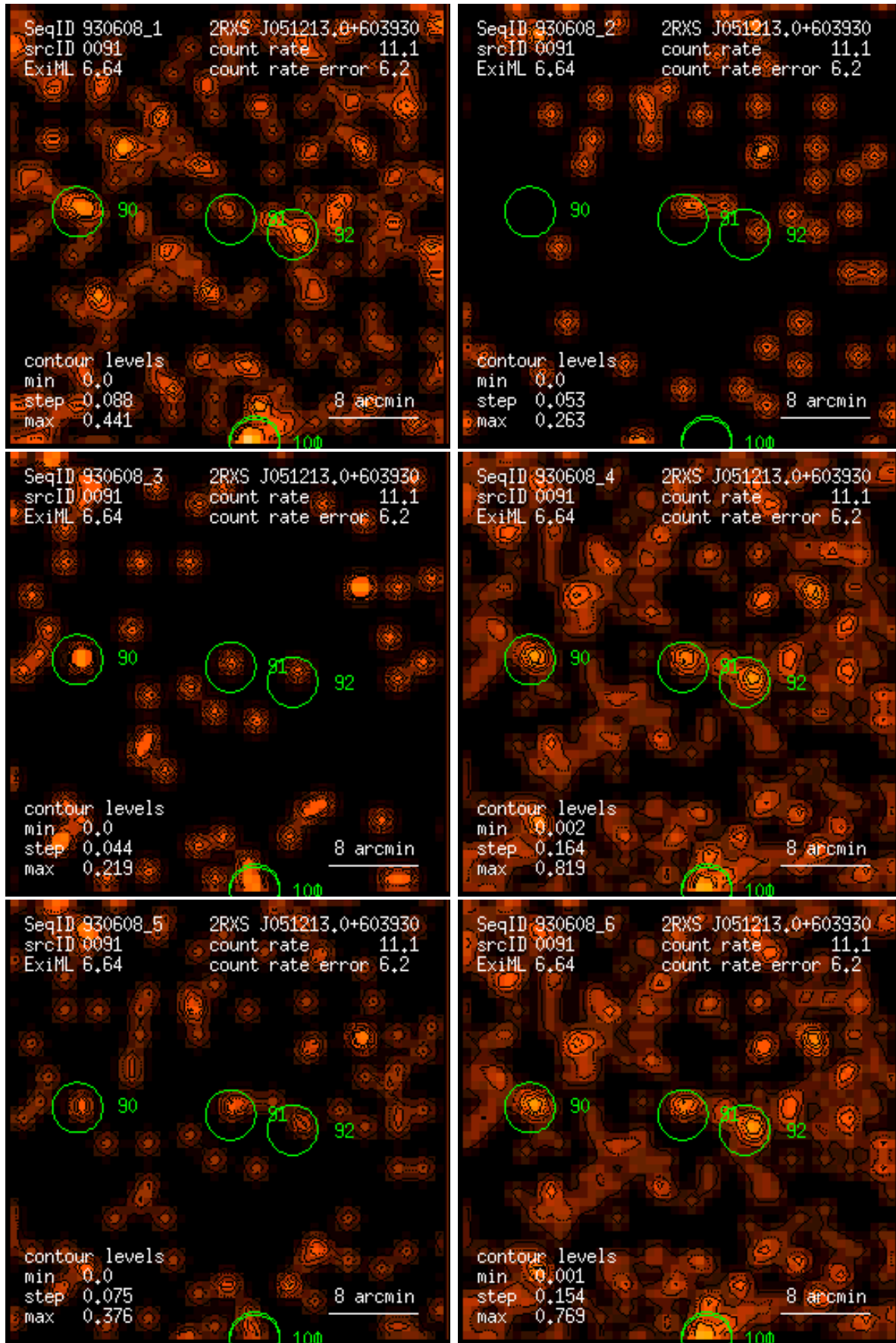
Figure 91: RASS 930608: detection 0091: band rate images, Gaussian filter: (1) PSPC channels 11 – 41, (2) 52 – 90, (3) 91 – 201, (4) 11 – 235, (5) 52 – 201, (6) 11 – 201. Broad band rates in counts/ks. Band rate contour levels in counts/ks/arcmin 2 .
