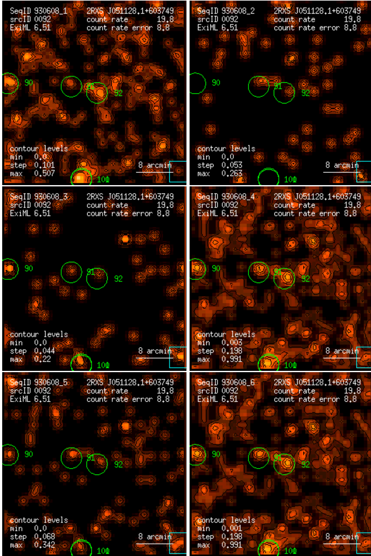
Figure 92: RASS 930608: detection 0092: band rate images, Gaussian filter: (1) PSPC channels 11 – 41, (2) 52 – 90, (3) 91 – 201, (4) 11 – 235, (5) 52 – 201, (6) 11 – 201. Broad band rates in counts/ks. Band rate contour levels in counts/ks/arcmin 2 .
