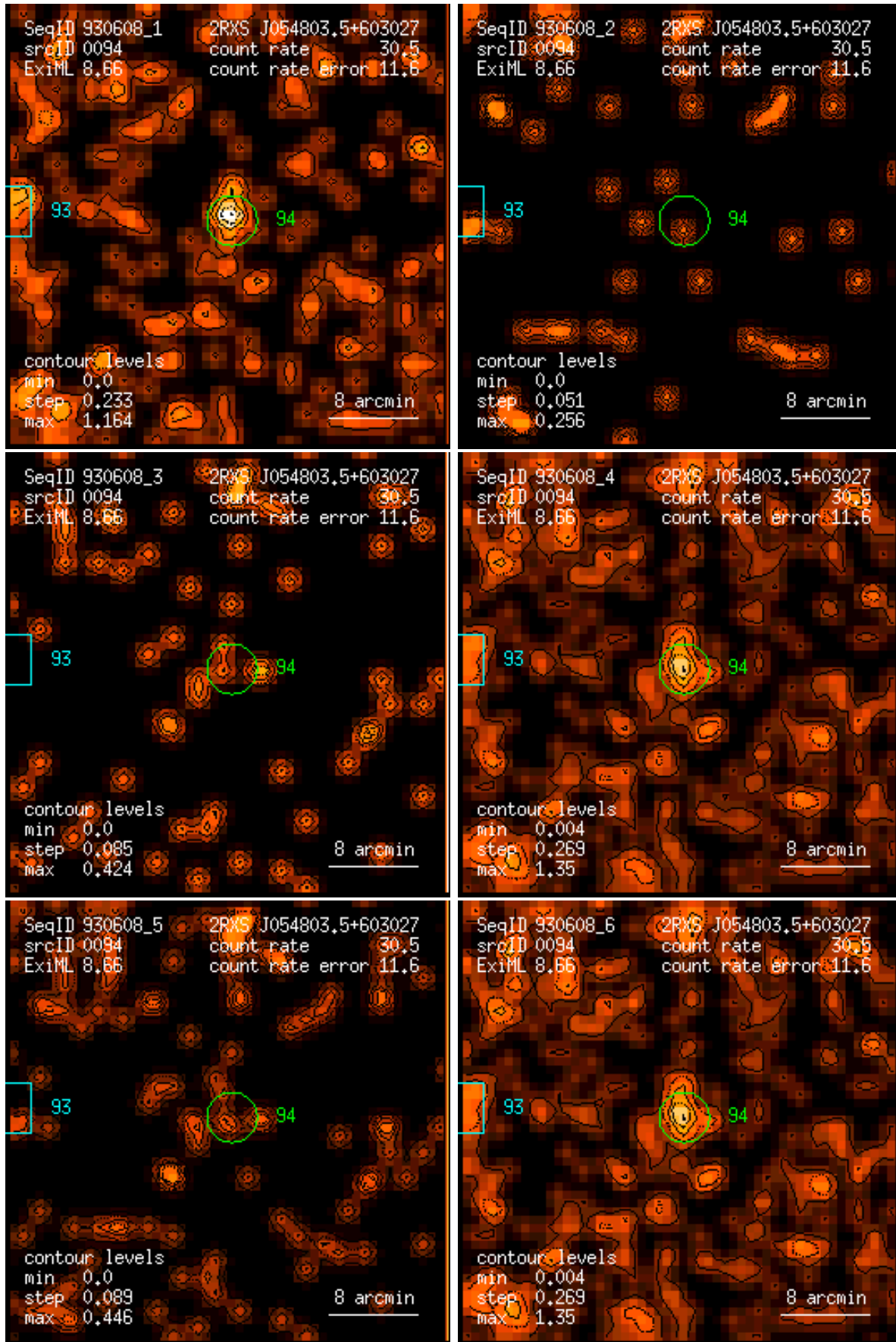
Figure 94: RASS 930608: detection 0094: band rate images, Gaussian filter: (1) PSPC channels 11 – 41, (2) 52 – 90, (3) 91 – 201, (4) 11 – 235, (5) 52 – 201, (6) 11 – 201. Broad band rates in counts/ks. Band rate contour levels in counts/ks/arcmin 2 .
