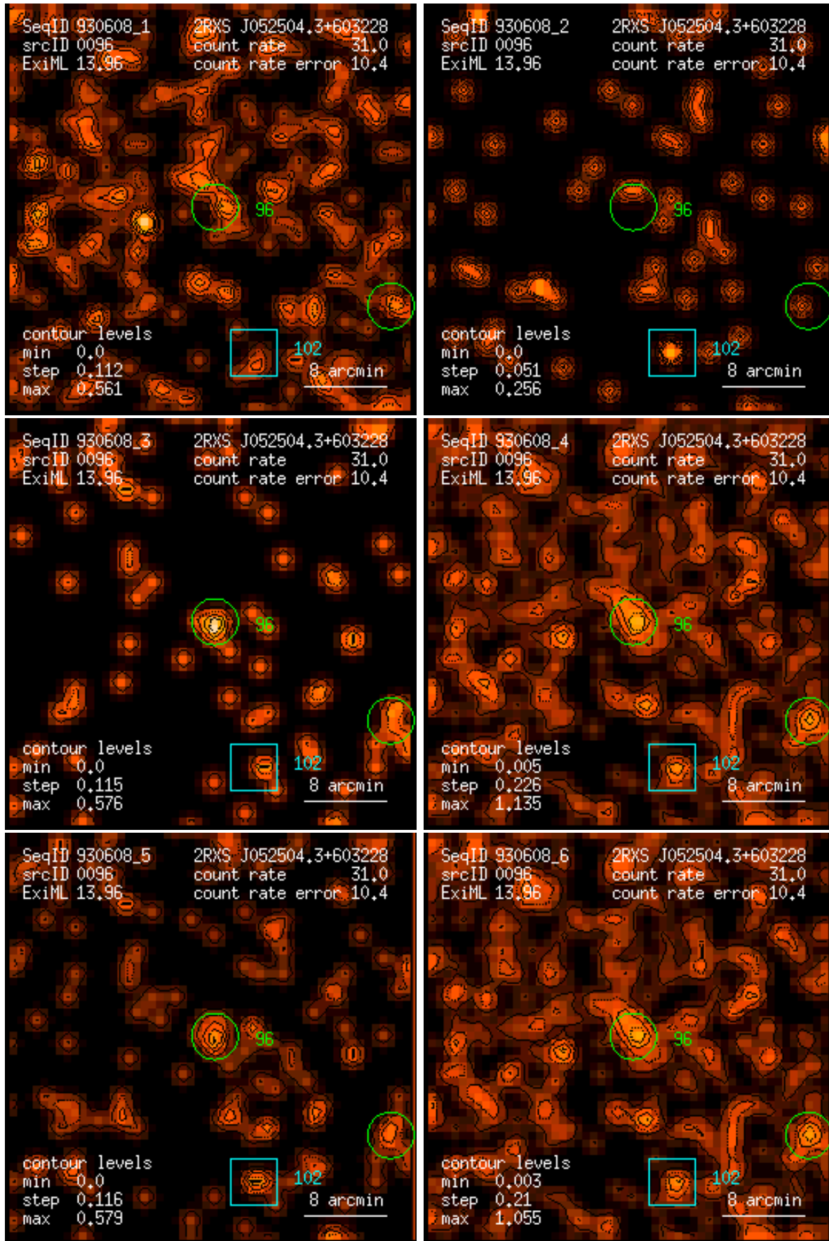
Figure 96: RASS 930608: detection 0096: band rate images, Gaussian filter: (1) PSPC channels 11 – 41, (2) 52 – 90, (3) 91 – 201, (4) 11 – 235, (5) 52 – 201, (6) 11 – 201. Broad band rates in counts/ks. Band rate contour levels in counts/ks/arcmin 2 .
