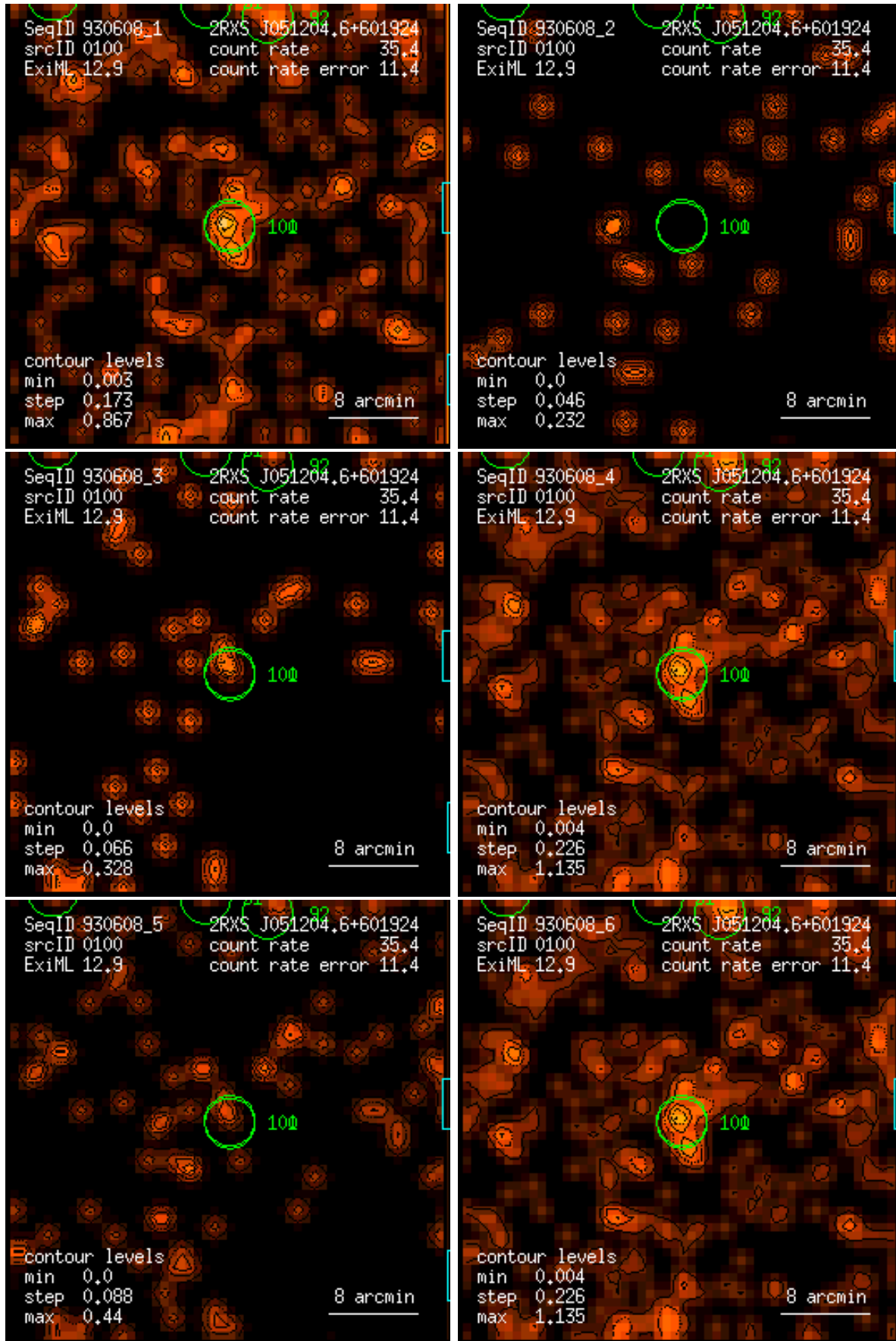
Figure 100: RASS 930608: detection 0100: band rate images, Gaussian filter: (1) PSPC channels 11 – 41, (2) 52 – 90, (3) 91 – 201, (4) 11 – 235, (5) 52 – 201, (6) 11 – 201. Broad band rates in counts/ks. Band rate contour levels in counts/ks/arcmin 2 .
