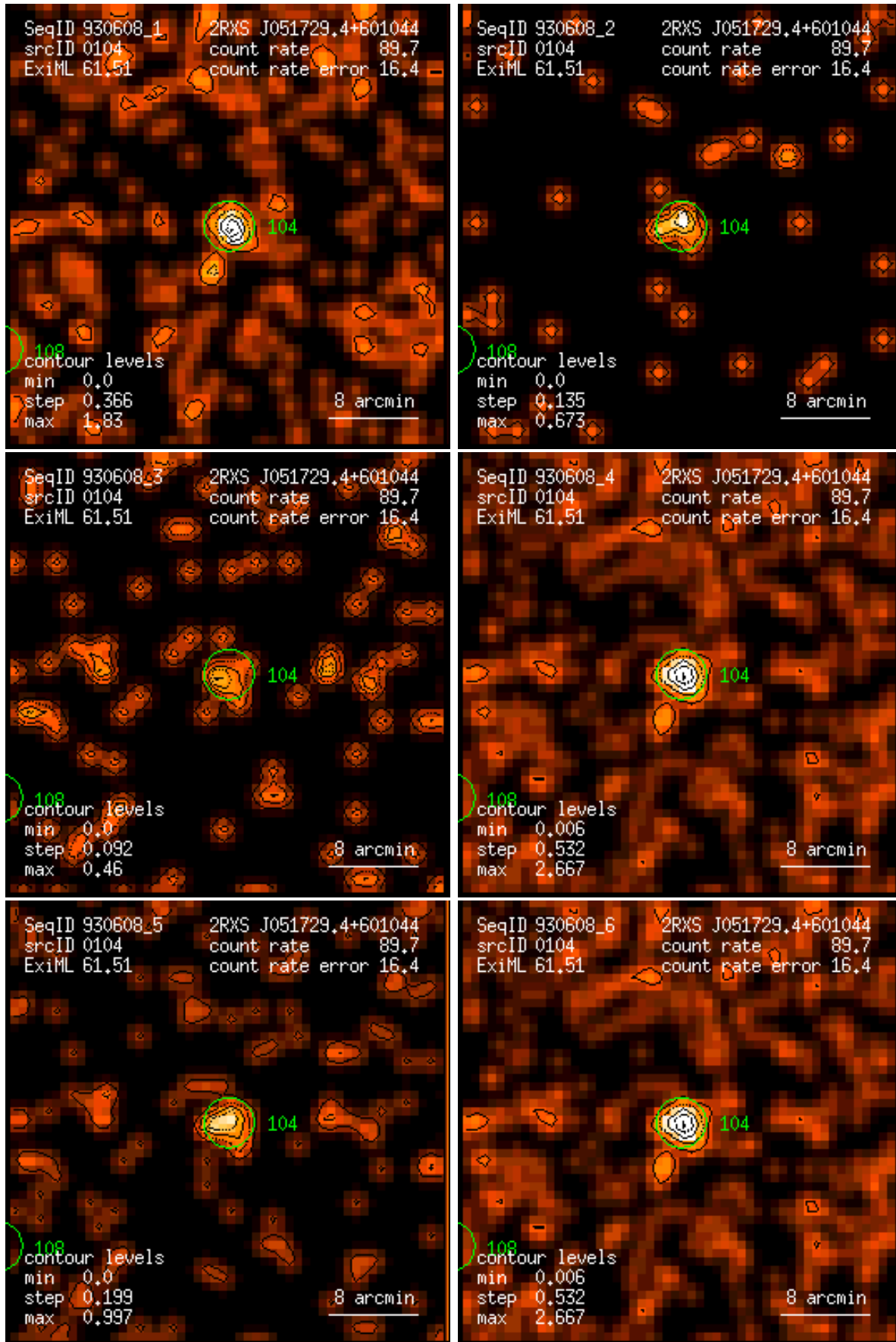
Figure 104: RASS 930608: detection 0104: band rate images, Gaussian filter: (1) PSPC channels 11 – 41, (2) 52 – 90, (3) 91 – 201, (4) 11 – 235, (5) 52 – 201, (6) 11 – 201. Broad band rates in counts/ks. Band rate contour levels in counts/ks/arcmin 2 .
