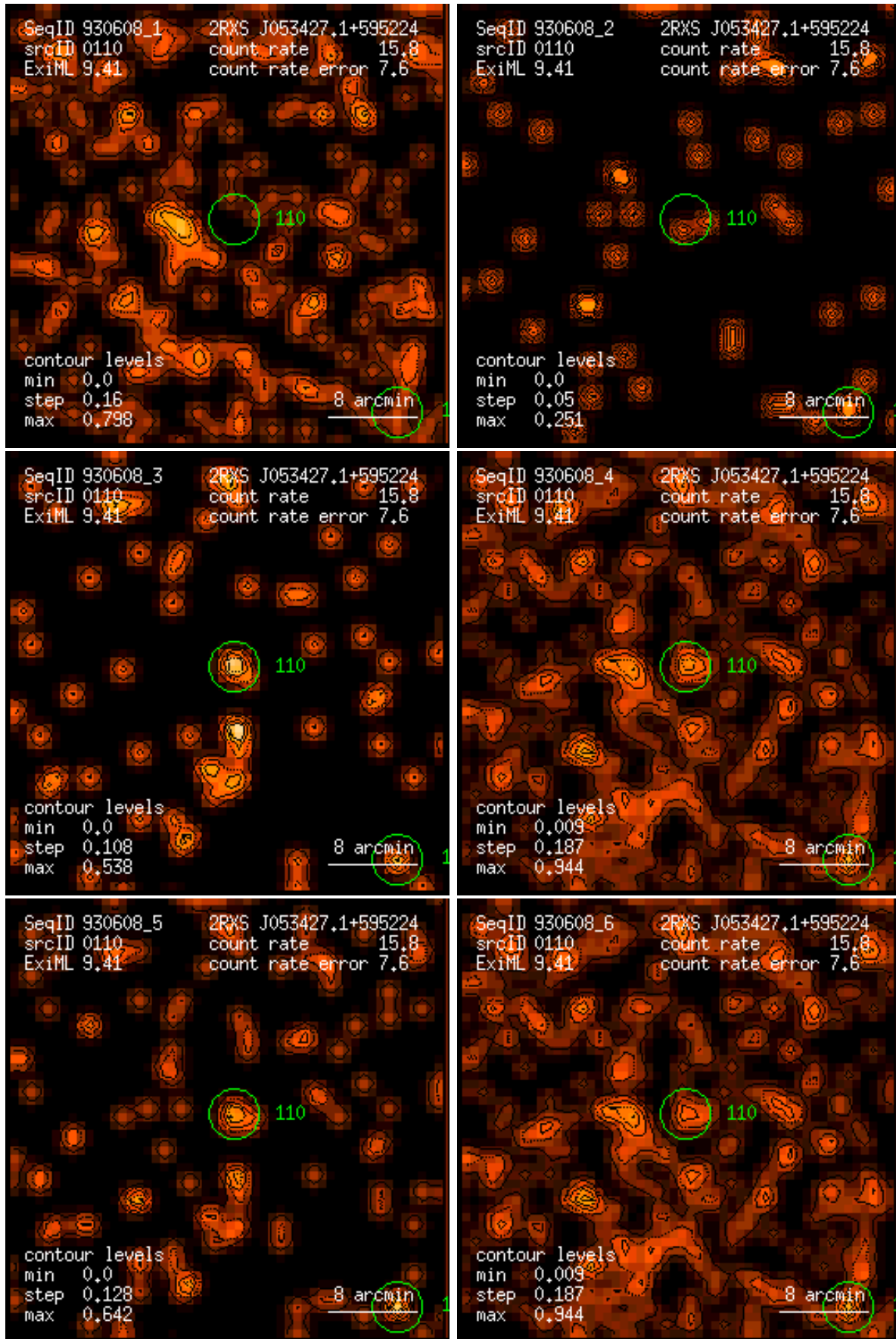
Figure 110: RASS 930608: detection 0110: band rate images, Gaussian filter: (1) PSPC channels 11 – 41, (2) 52 – 90, (3) 91 – 201, (4) 11 – 235, (5) 52 – 201, (6) 11 – 201. Broad band rates in counts/ks. Band rate contour levels in counts/ks/arcmin 2 .
