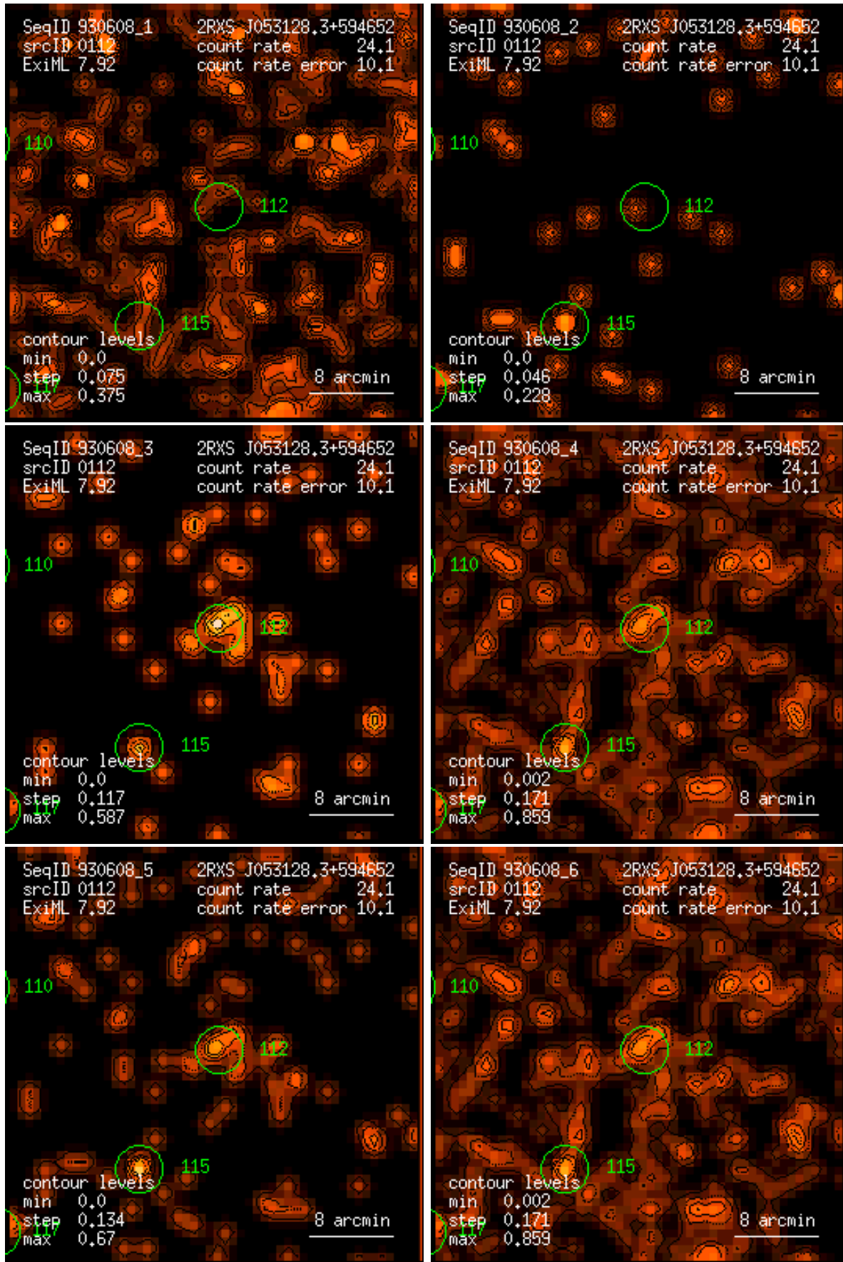
Figure 112: RASS 930608: detection 0112: band rate images, Gaussian filter: (1) PSPC channels 11 – 41, (2) 52 – 90, (3) 91 – 201, (4) 11 – 235, (5) 52 – 201, (6) 11 – 201. Broad band rates in counts/ks. Band rate contour levels in counts/ks/arcmin 2 .
