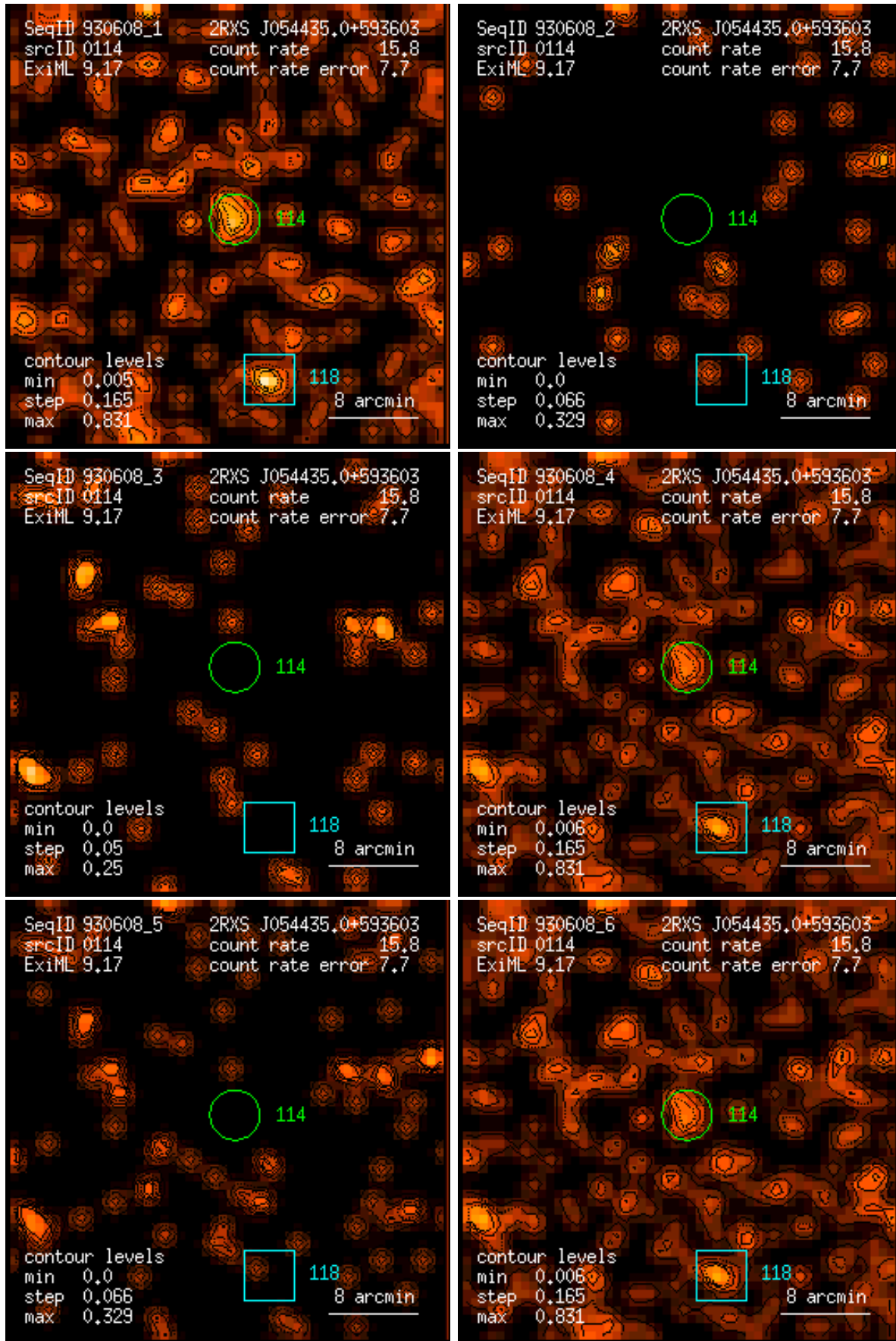
Figure 114: RASS 930608: detection 0114: band rate images, Gaussian filter: (1) PSPC channels 11 – 41, (2) 52 – 90, (3) 91 – 201, (4) 11 – 235, (5) 52 – 201, (6) 11 – 201. Broad band rates in counts/ks. Band rate contour levels in counts/ks/arcmin 2 .
