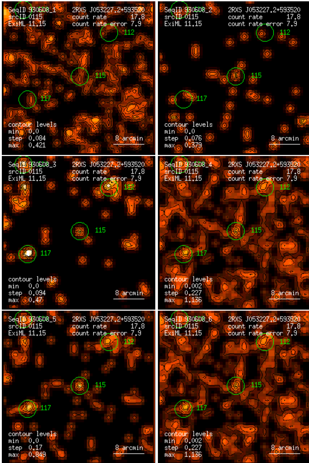
Figure 115: RASS 930608: detection 0115: band rate images, Gaussian filter: (1) PSPC channels 11 – 41, (2) 52 – 90, (3) 91 – 201, (4) 11 – 235, (5) 52 – 201, (6) 11 – 201. Broad band rates in counts/ks. Band rate contour levels in counts/ks/arcmin 2 .
