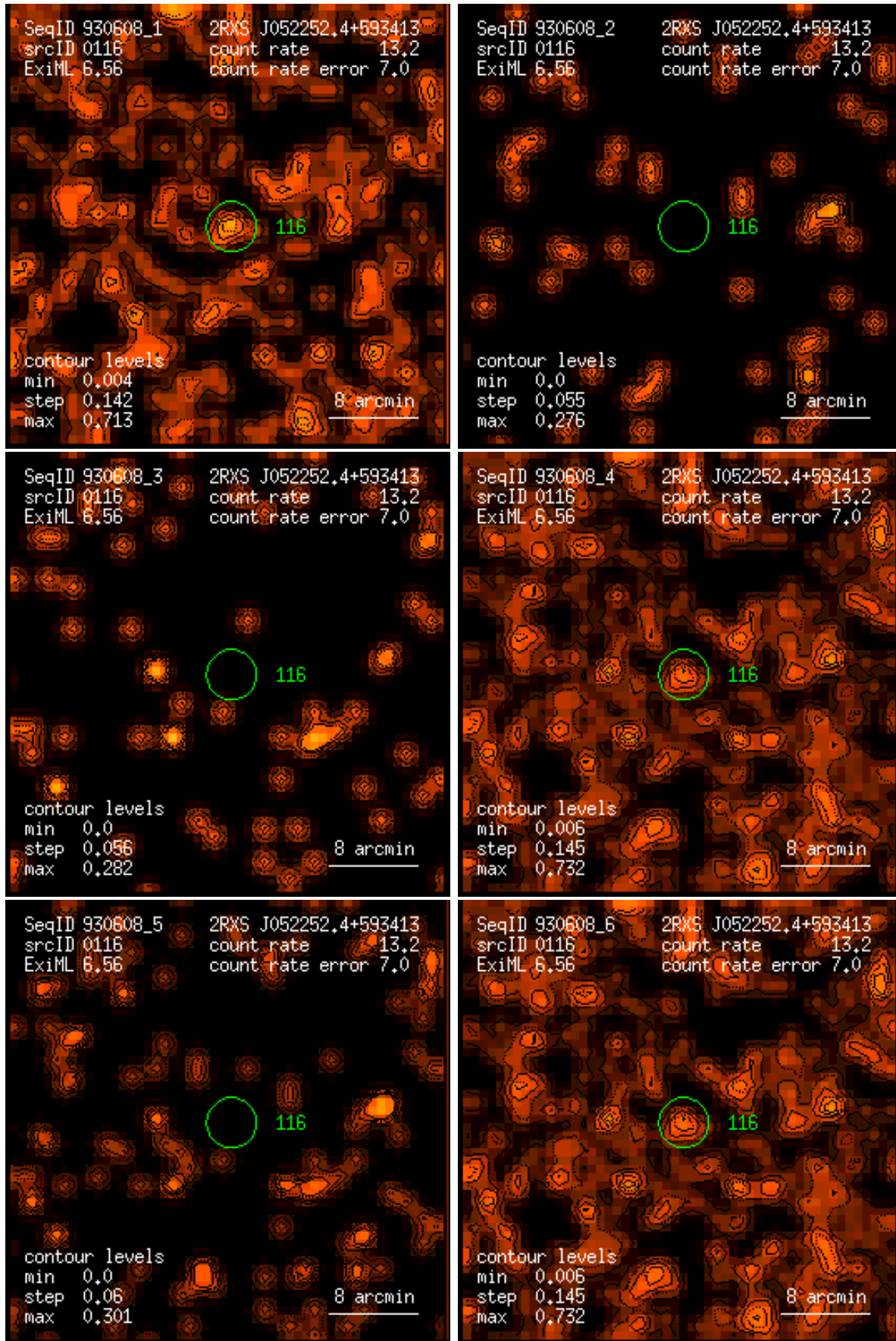
Figure 116: RASS 930608: detection 0116: band rate images, Gaussian filter: (1) PSPC channels 11 – 41, (2) 52 – 90, (3) 91 – 201, (4) 11 – 235, (5) 52 – 201, (6) 11 – 201. Broad band rates in counts/ks. Band rate contour levels in counts/ks/arcmin 2 .
