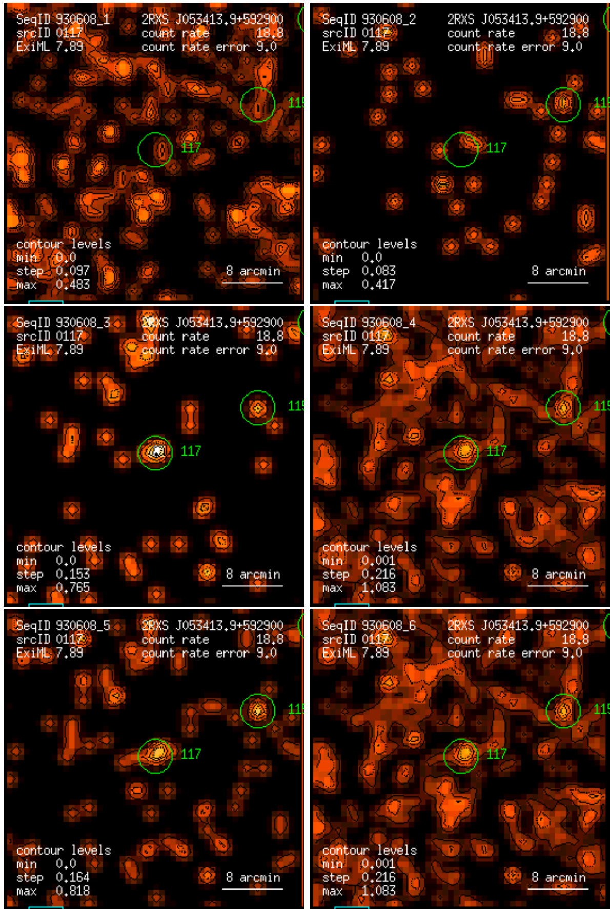
Figure 117: RASS 930608: detection 0117: band rate images, Gaussian filter: (1) PSPC channels 11 – 41, (2) 52 – 90, (3) 91 – 201, (4) 11 – 235, (5) 52 – 201, (6) 11 – 201. Broad band rates in counts/ks. Band rate contour levels in counts/ks/arcmin 2 .
