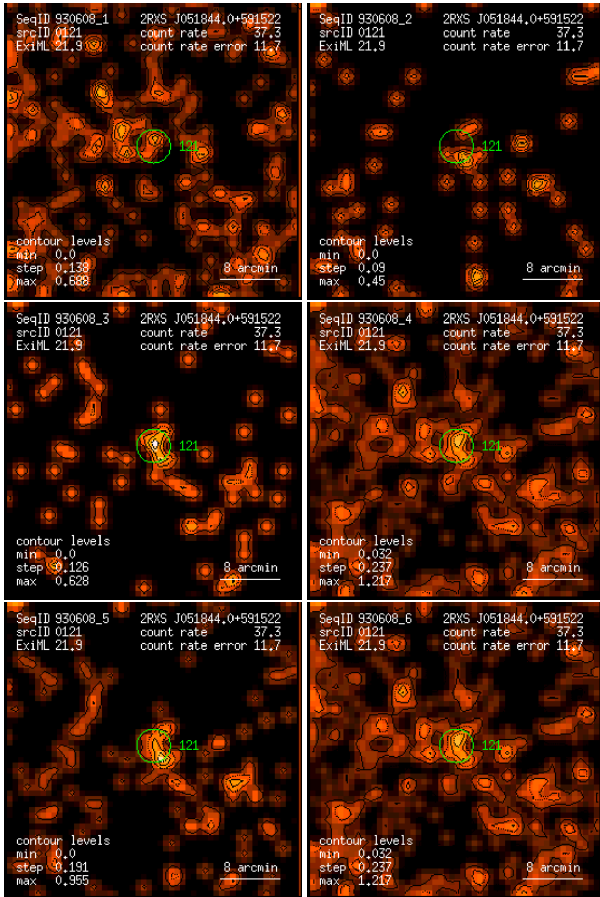
Figure 121: RASS 930608: detection 0121: band rate images, Gaussian filter: (1) PSPC channels 11 – 41, (2) 52 – 90, (3) 91 – 201, (4) 11 – 235, (5) 52 – 201, (6) 11 – 201. Broad band rates in counts/ks. Band rate contour levels in counts/ks/arcmin 2 .
