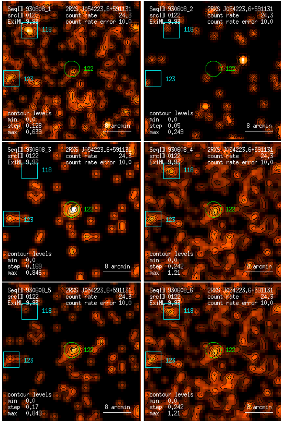
Figure 122: RASS 930608: detection 0122: band rate images, Gaussian filter: (1) PSPC channels 11 – 41, (2) 52 – 90, (3) 91 – 201, (4) 11 – 235, (5) 52 – 201, (6) 11 – 201. Broad band rates in counts/ks. Band rate contour levels in counts/ks/arcmin 2 .
