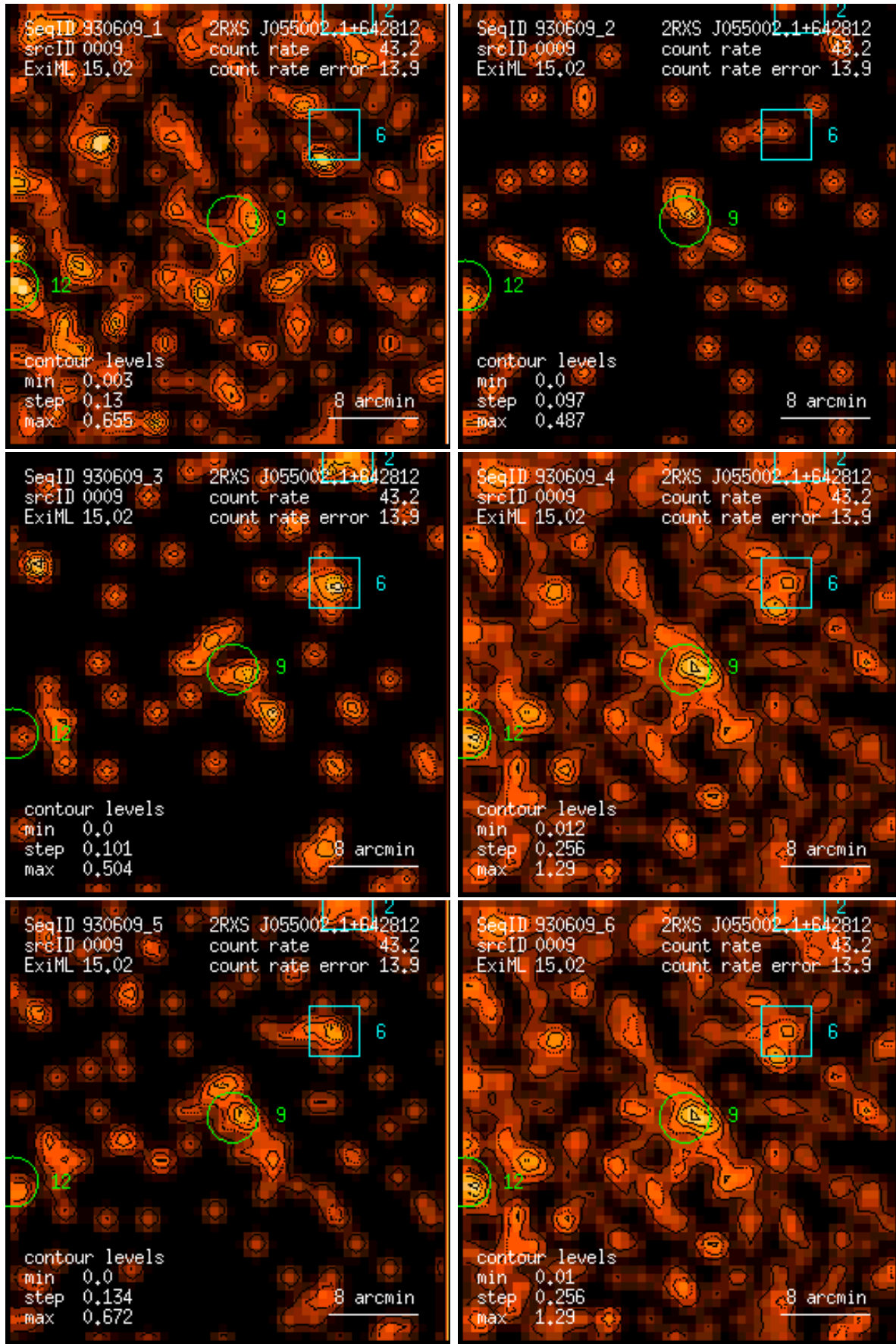
Figure 9: RASS 930609: detection 0009: band rate images, Gaussian filter: (1) PSPC channels 11 – 41, (2) 52 – 90, (3) 91 – 201, (4) 11 – 235, (5) 52 – 201, (6) 11 – 201. Broad band rates in counts/ks. Band rate contour levels in counts/ks/arcmin 2 .
