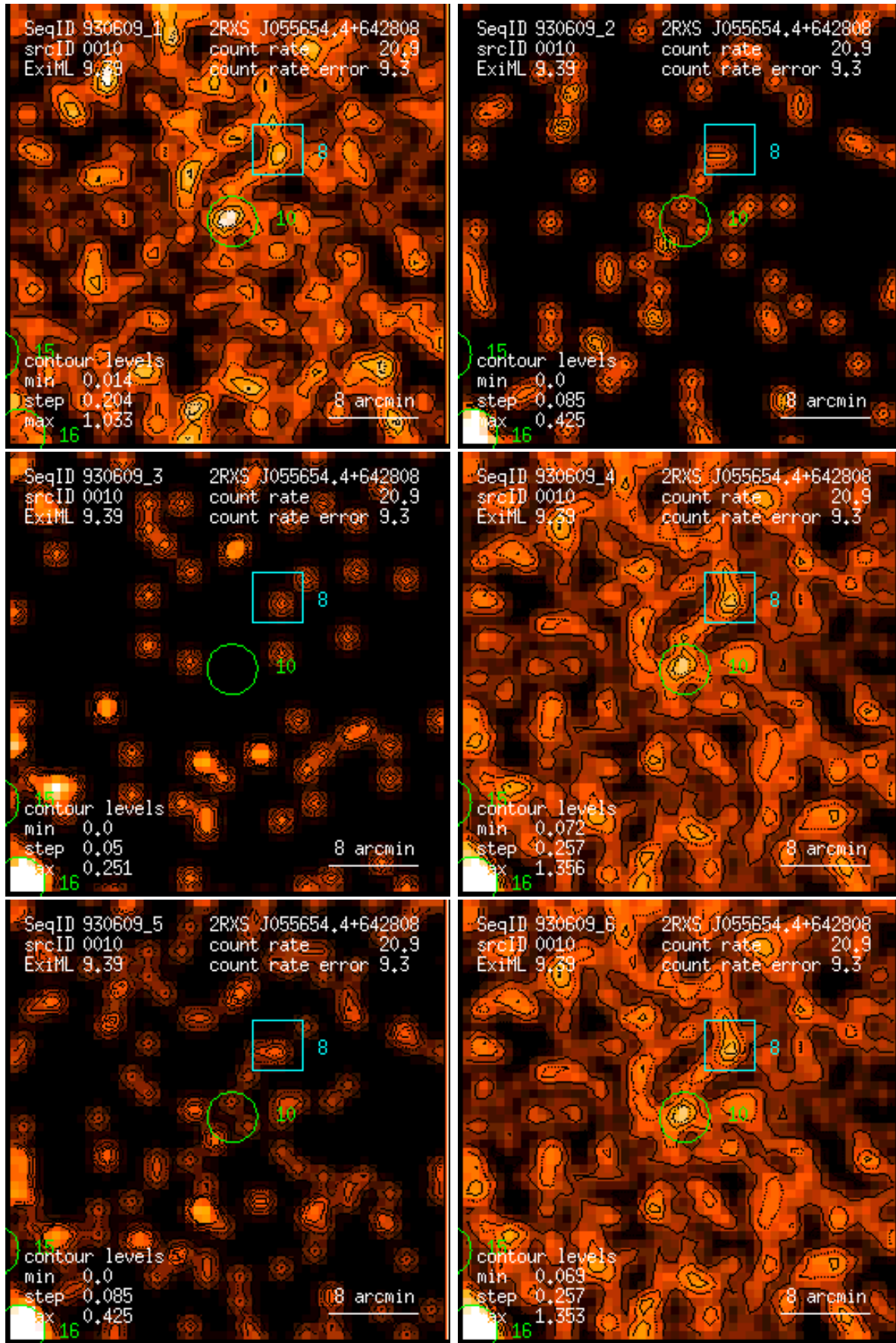
Figure 10: RASS 930609: detection 0010: band rate images, Gaussian filter: (1) PSPC channels 11 – 41, (2) 52 – 90, (3) 91 – 201, (4) 11 – 235, (5) 52 – 201, (6) 11 – 201. Broad band rates in counts/ks. Band rate contour levels in counts/ks/arcmin 2 .
