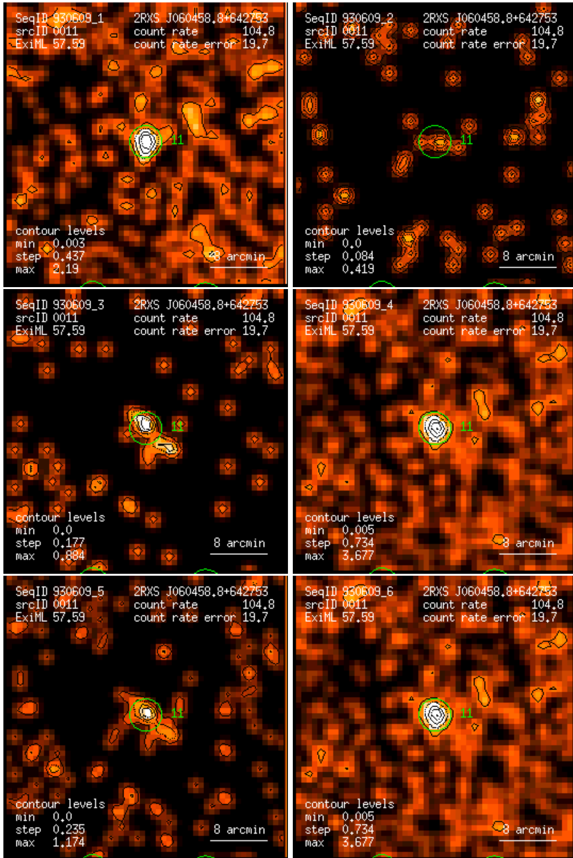
Figure 11: RASS 930609: detection 0011: band rate images, Gaussian filter: (1) PSPC channels 11 – 41, (2) 52 – 90, (3) 91 – 201, (4) 11 – 235, (5) 52 – 201, (6) 11 – 201. Broad band rates in counts/ks. Band rate contour levels in counts/ks/arcmin 2 .
