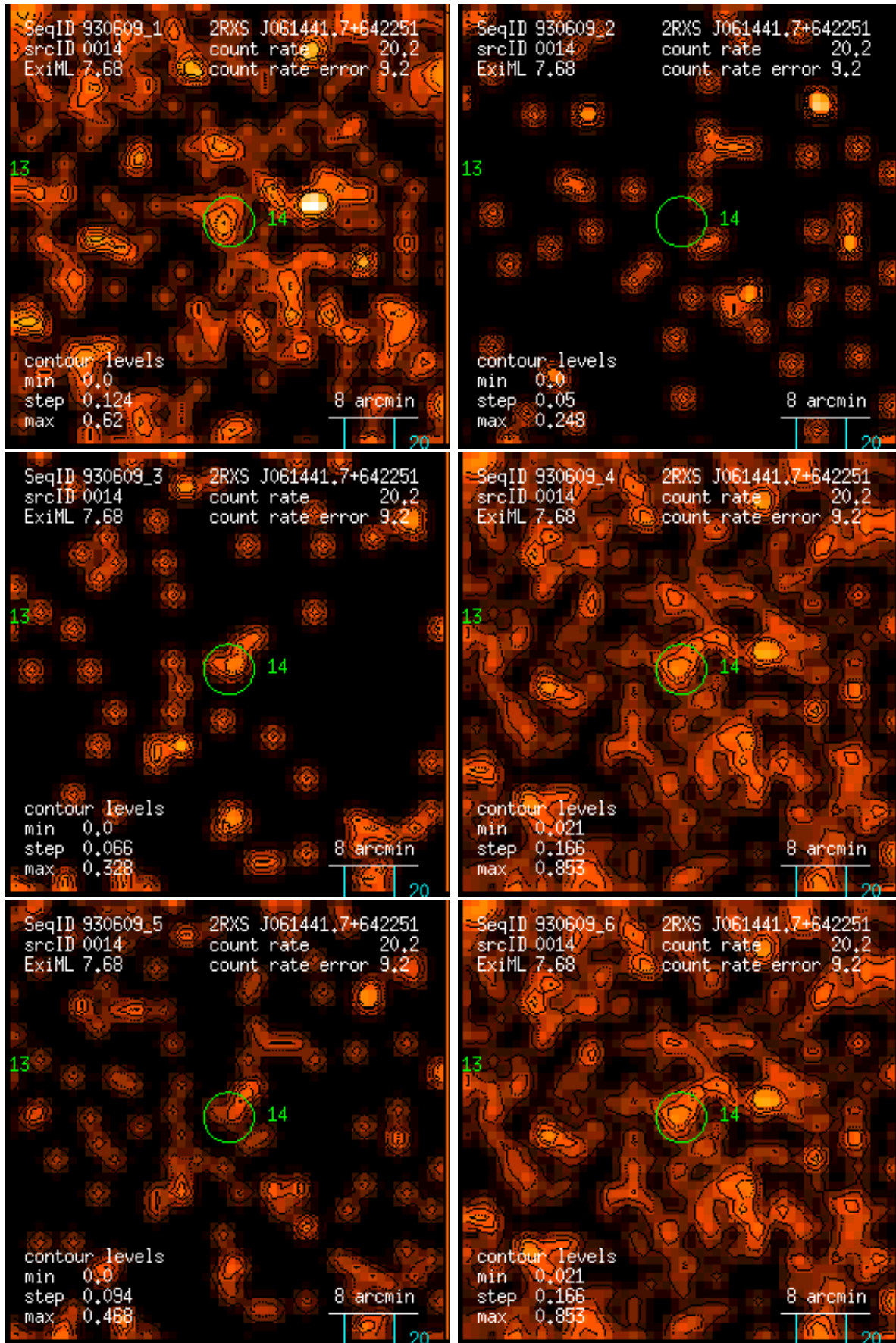
Figure 14: RASS 930609: detection 0014: band rate images, Gaussian filter: (1) PSPC channels 11 – 41, (2) 52 – 90, (3) 91 – 201, (4) 11 – 235, (5) 52 – 201, (6) 11 – 201. Broad band rates in counts/ks. Band rate contour levels in counts/ks/arcmin 2 .
