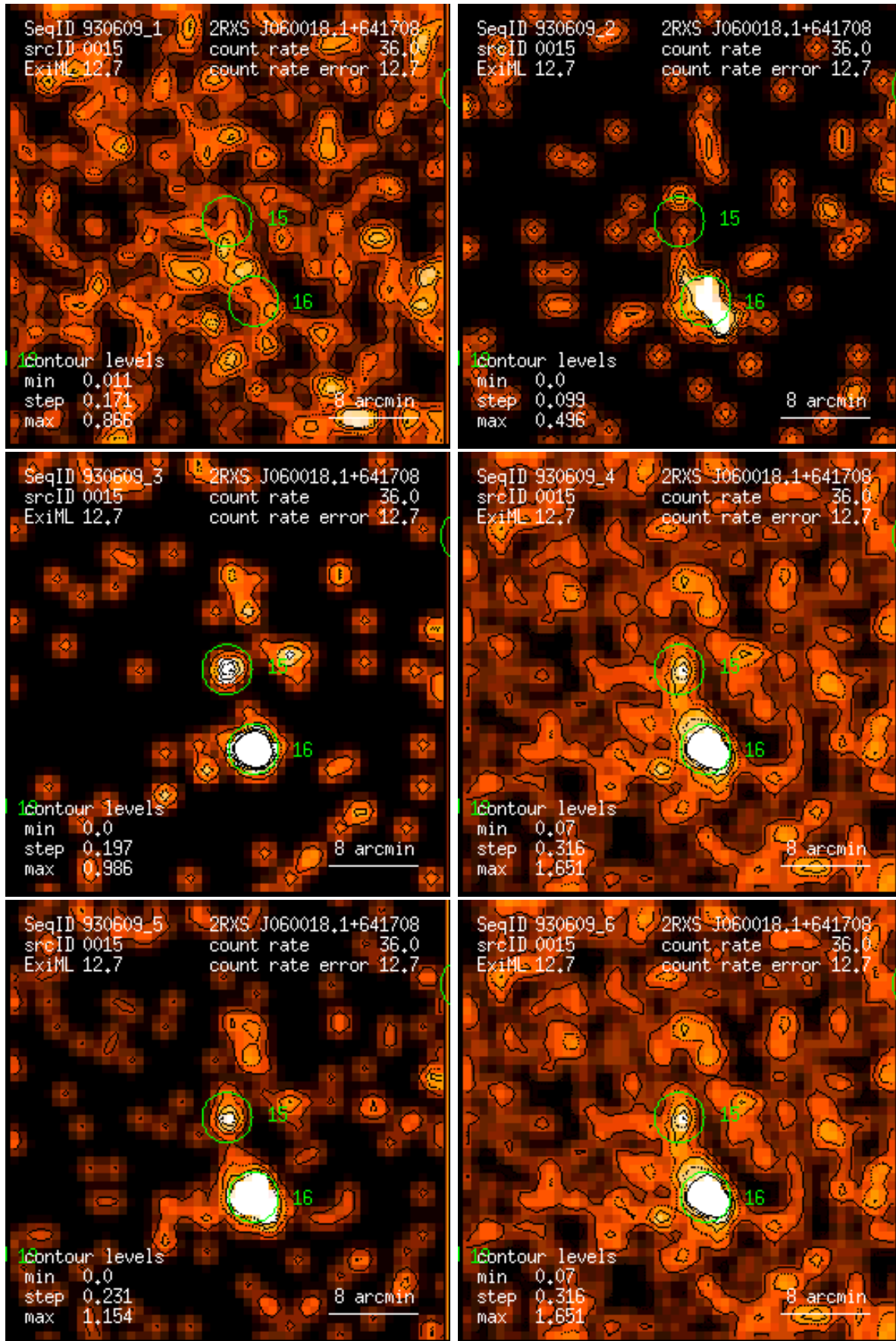
Figure 15: RASS 930609: detection 0015: band rate images, Gaussian filter: (1) PSPC channels 11 – 41, (2) 52 – 90, (3) 91 – 201, (4) 11 – 235, (5) 52 – 201, (6) 11 – 201. Broad band rates in counts/ks. Band rate contour levels in counts/ks/arcmin 2 .
