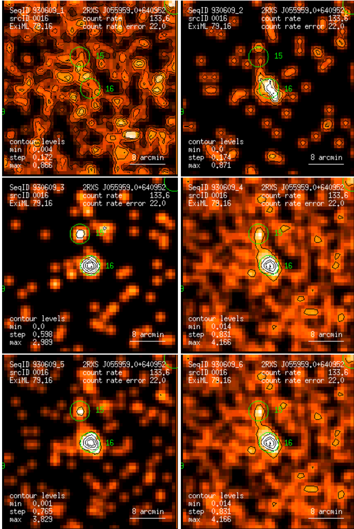
Figure 16: RASS 930609: detection 0016: band rate images, Gaussian filter: (1) PSPC channels 11 – 41, (2) 52 – 90, (3) 91 – 201, (4) 11 – 235, (5) 52 – 201, (6) 11 – 201. Broad band rates in counts/ks. Band rate contour levels in counts/ks/arcmin 2 .
