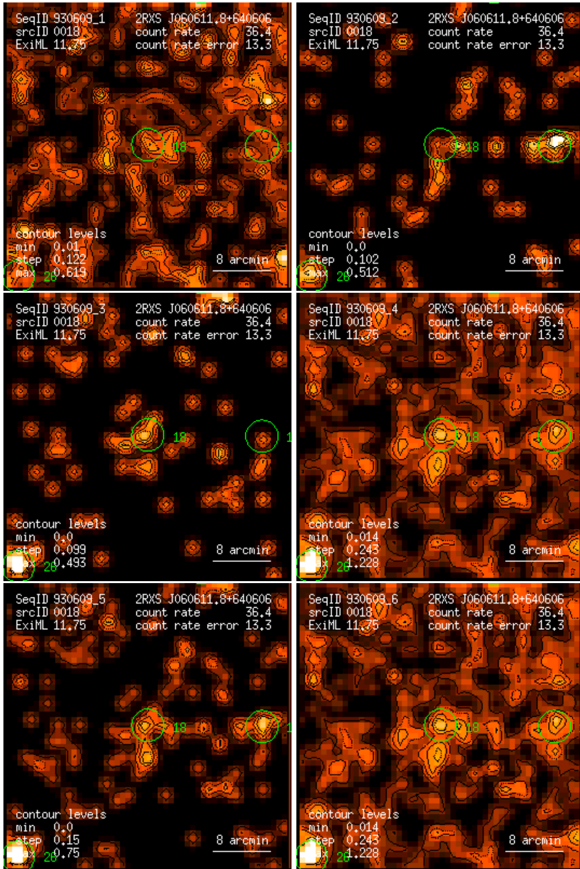
Figure 18: RASS 930609: detection 0018: band rate images, Gaussian filter: (1) PSPC channels 11 – 41, (2) 52 – 90, (3) 91 – 201, (4) 11 – 235, (5) 52 – 201, (6) 11 – 201. Broad band rates in counts/ks. Band rate contour levels in counts/ks/arcmin 2 .
