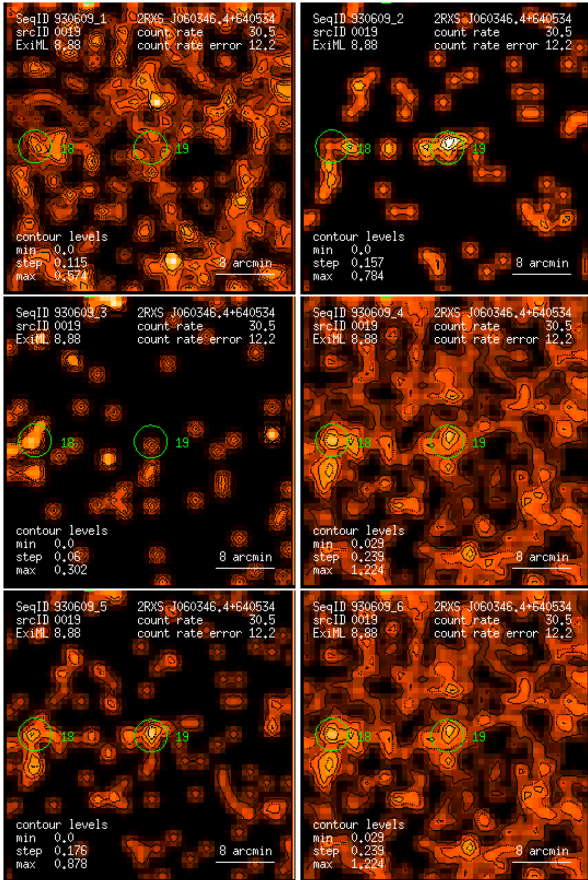
Figure 19: RASS 930609: detection 0019: band rate images, Gaussian filter: (1) PSPC channels 11 – 41, (2) 52 – 90, (3) 91 – 201, (4) 11 – 235, (5) 52 – 201, (6) 11 – 201. Broad band rates in counts/ks. Band rate contour levels in counts/ks/arcmin 2 .
