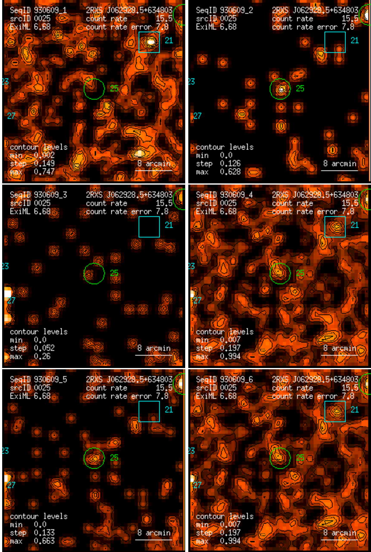
Figure 25: RASS 930609: detection 0025: band rate images, Gaussian filter: (1) PSPC channels 11 – 41, (2) 52 – 90, (3) 91 – 201, (4) 11 – 235, (5) 52 – 201, (6) 11 – 201. Broad band rates in counts/ks. Band rate contour levels in counts/ks/arcmin 2 .
