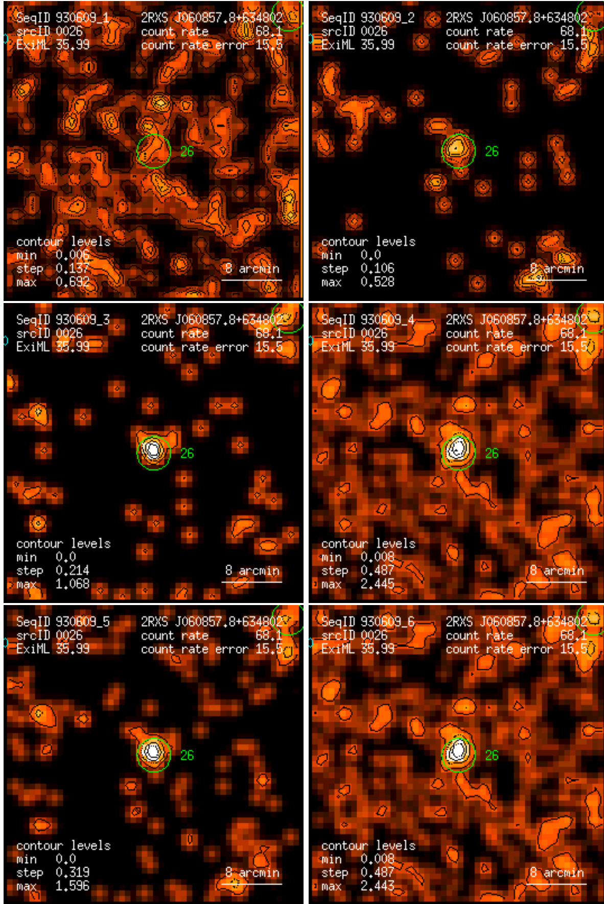
Figure 26: RASS 930609: detection 0026: band rate images, Gaussian filter: (1) PSPC channels 11 – 41, (2) 52 – 90, (3) 91 – 201, (4) 11 – 235, (5) 52 – 201, (6) 11 – 201. Broad band rates in counts/ks. Band rate contour levels in counts/ks/arcmin 2 .
