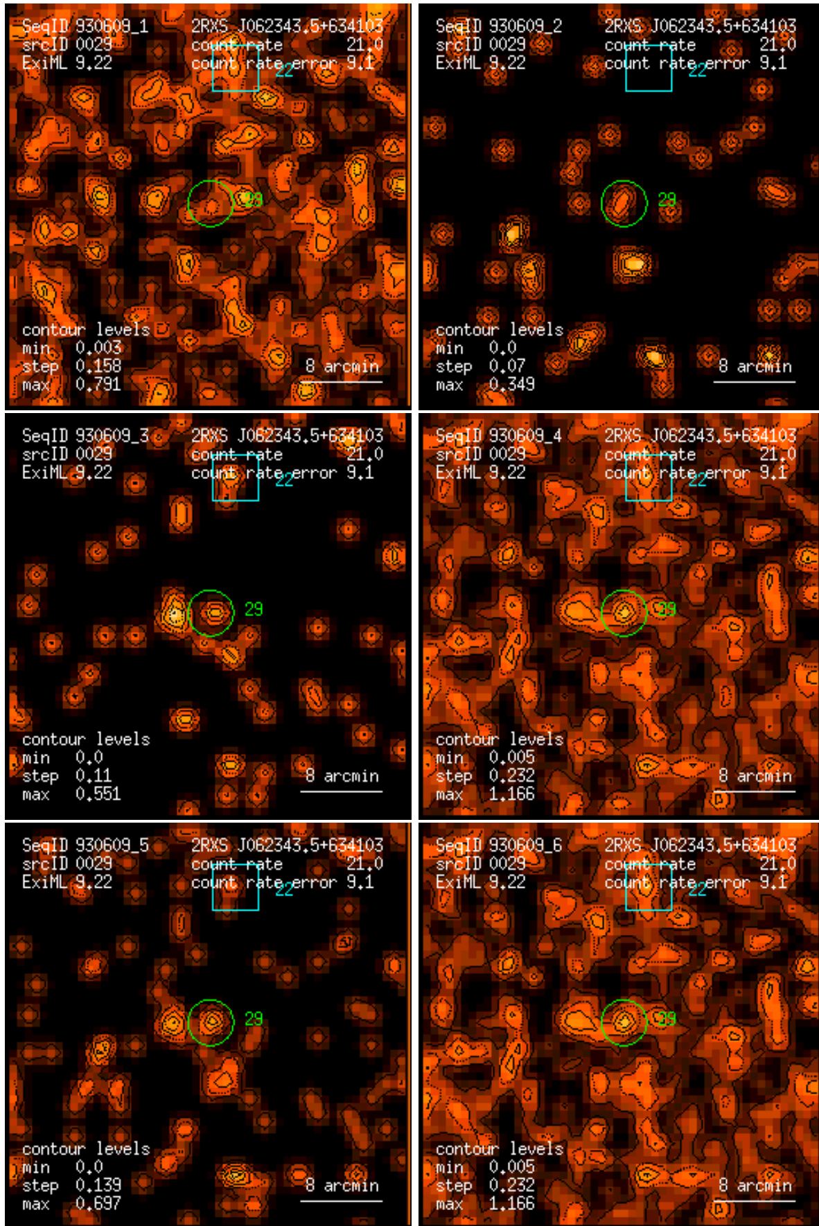
Figure 29: RASS 930609: detection 0029: band rate images, Gaussian filter: (1) PSPC channels 11 – 41, (2) 52 – 90, (3) 91 – 201, (4) 11 – 235, (5) 52 – 201, (6) 11 – 201. Broad band rates in counts/ks. Band rate contour levels in counts/ks/arcmin 2 .
