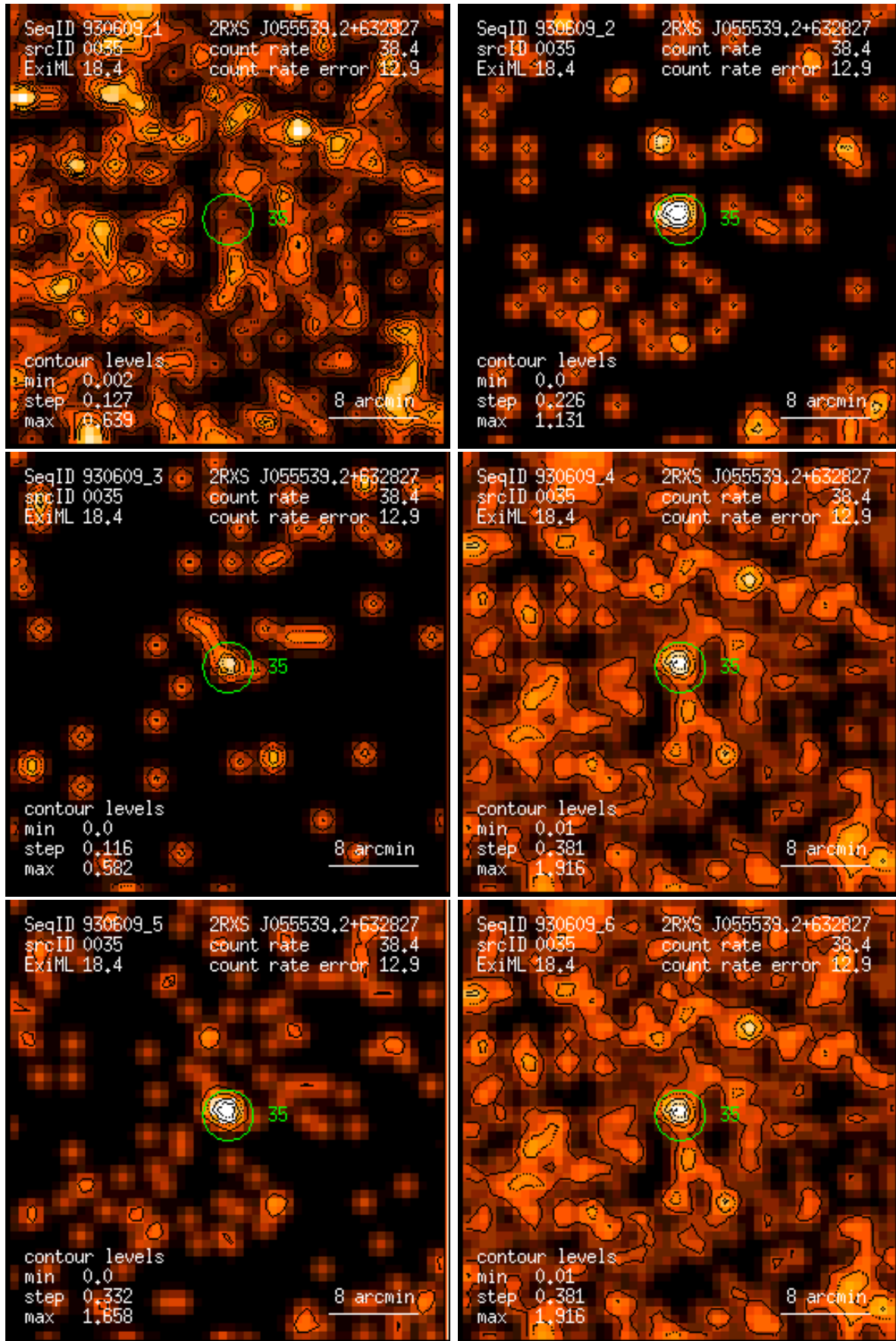
Figure 35: RASS 930609: detection 0035: band rate images, Gaussian filter: (1) PSPC channels 11 – 41, (2) 52 – 90, (3) 91 – 201, (4) 11 – 235, (5) 52 – 201, (6) 11 – 201. Broad band rates in counts/ks. Band rate contour levels in counts/ks/arcmin 2 .
