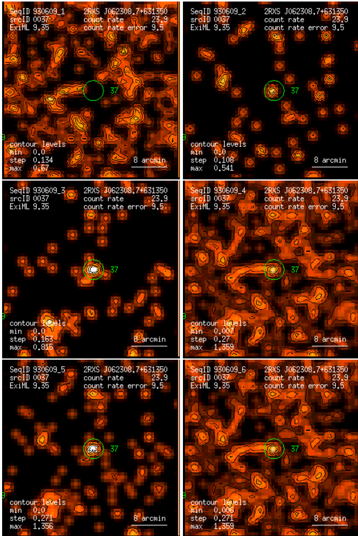
Figure 37: RASS 930609: detection 0037: band rate images, Gaussian filter: (1) PSPC channels 11 – 41, (2) 52 – 90, (3) 91 – 201, (4) 11 – 235, (5) 52 – 201, (6) 11 – 201. Broad band rates in counts/ks. Band rate contour levels in counts/ks/arcmin 2 .
